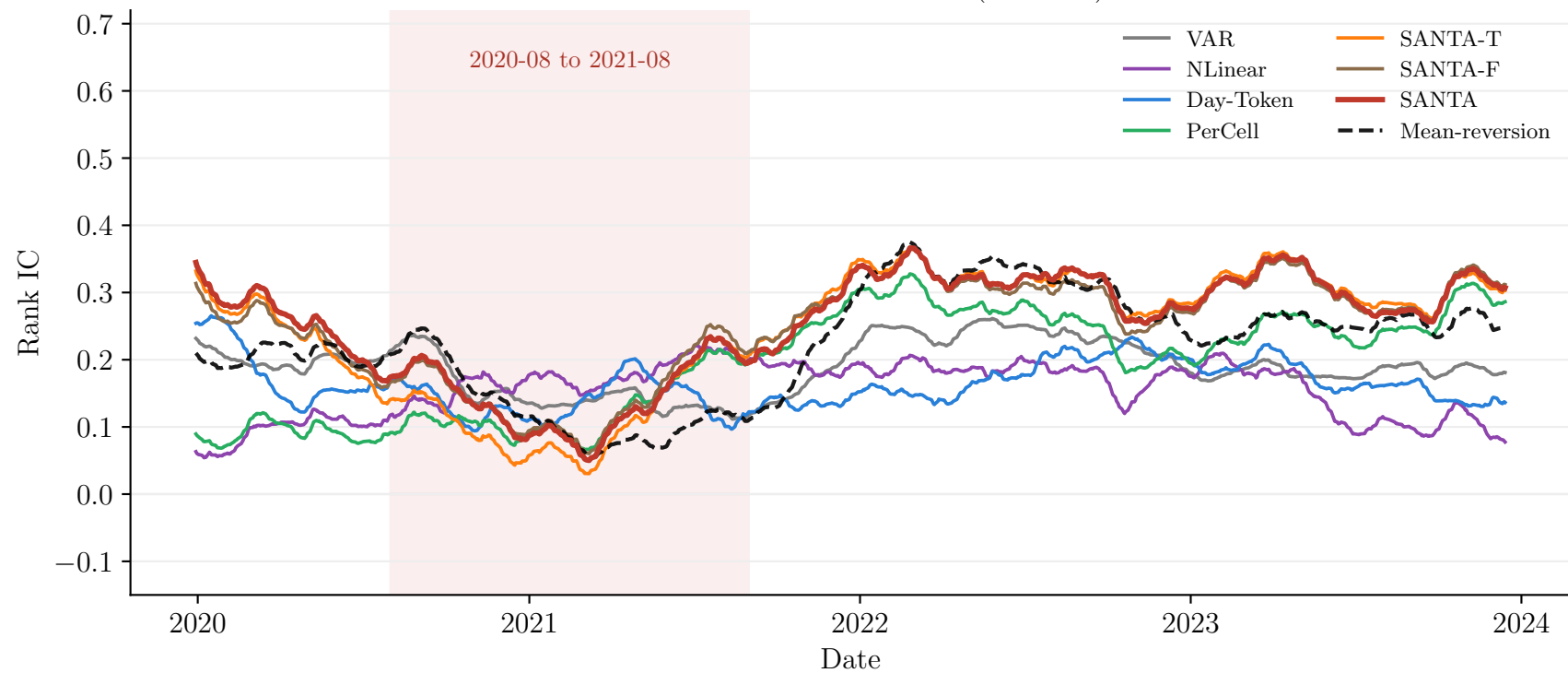
Forecast rank IC: full test set (MA: 252)
