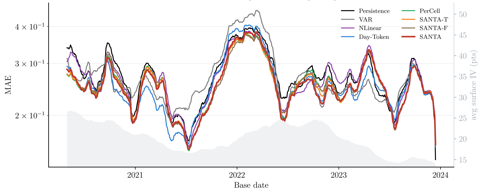
Forecast MAE from May 2020 onwards (MA-63)
