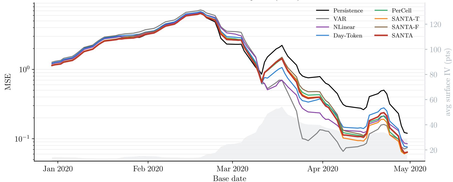
Forecast MSE: COVID-19 period (MA-5)
