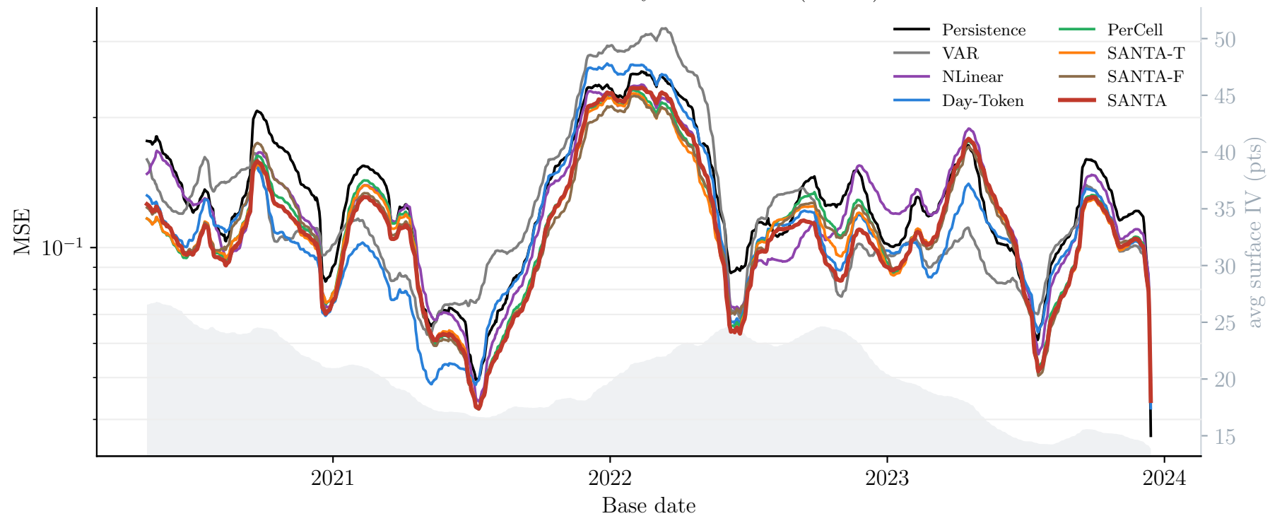
Forecast MSE from May 2020 onwards (MA-63)
