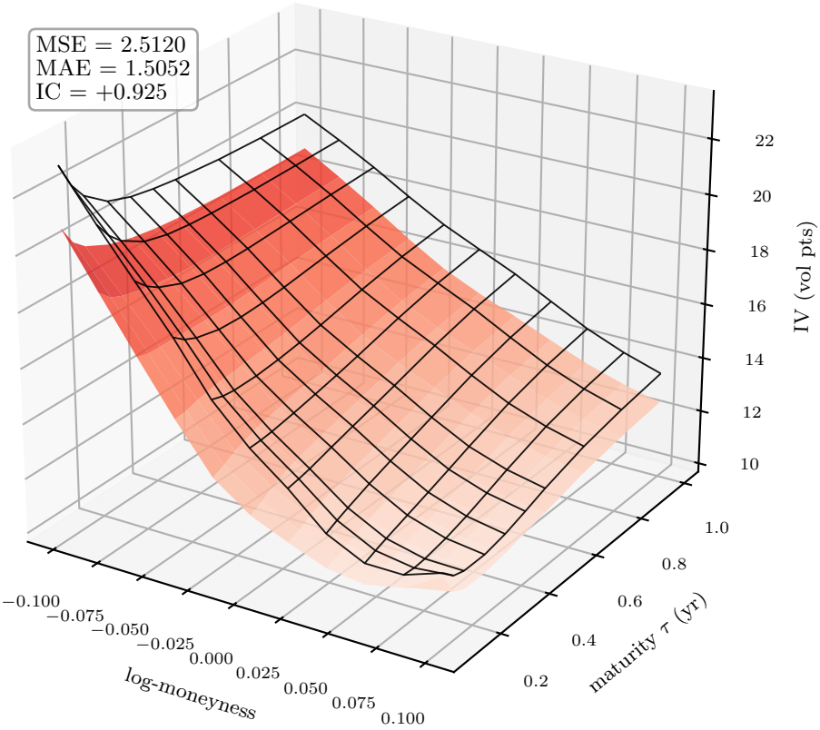
SANTA
