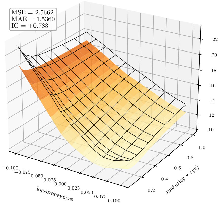
SANTA-Flat
