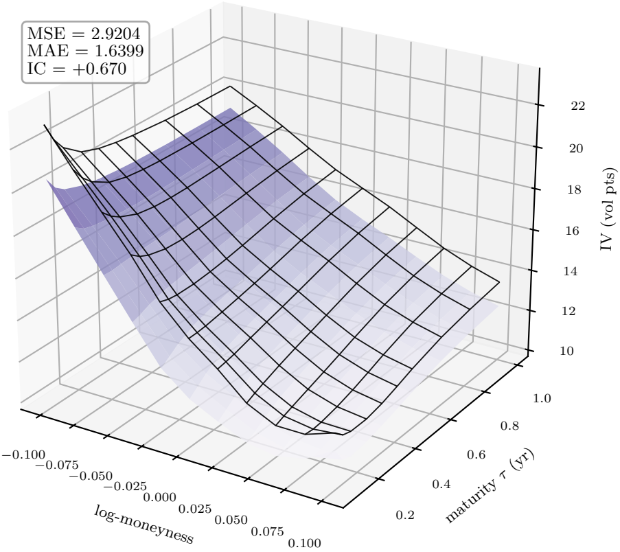
NLinear
