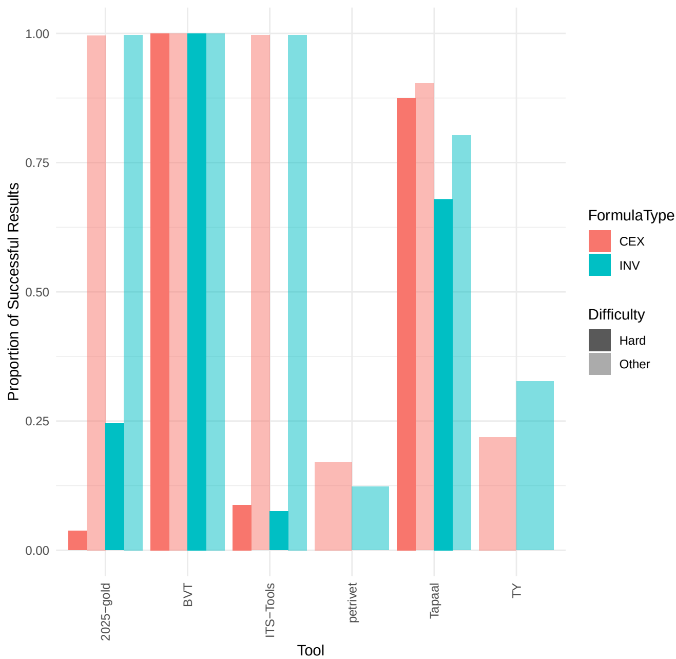
Performance of Main Tools for global_properties in 2026
