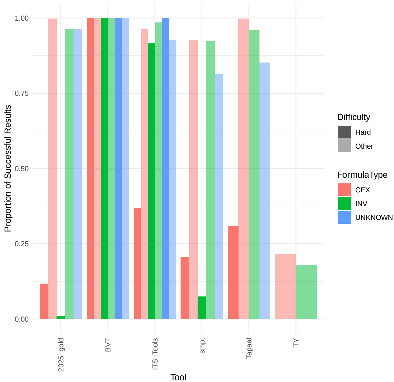
Performance of Main Tools for reachability in 2026
