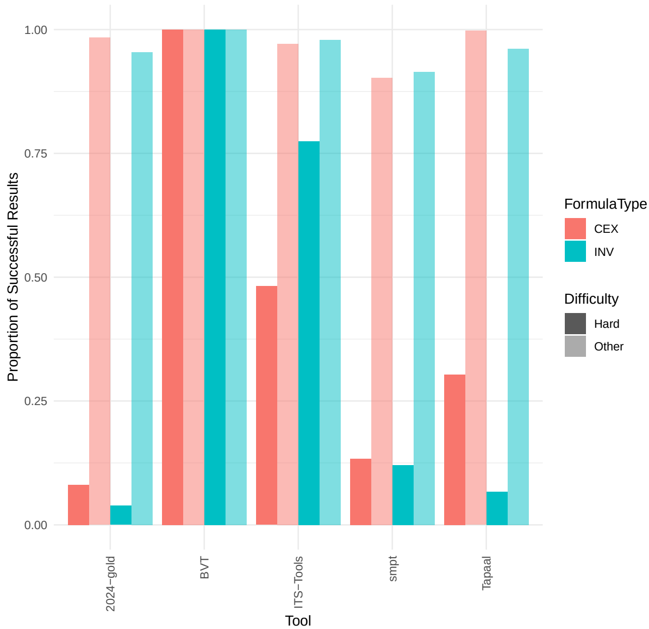
Performance of Main Tools for reachability in 2025
