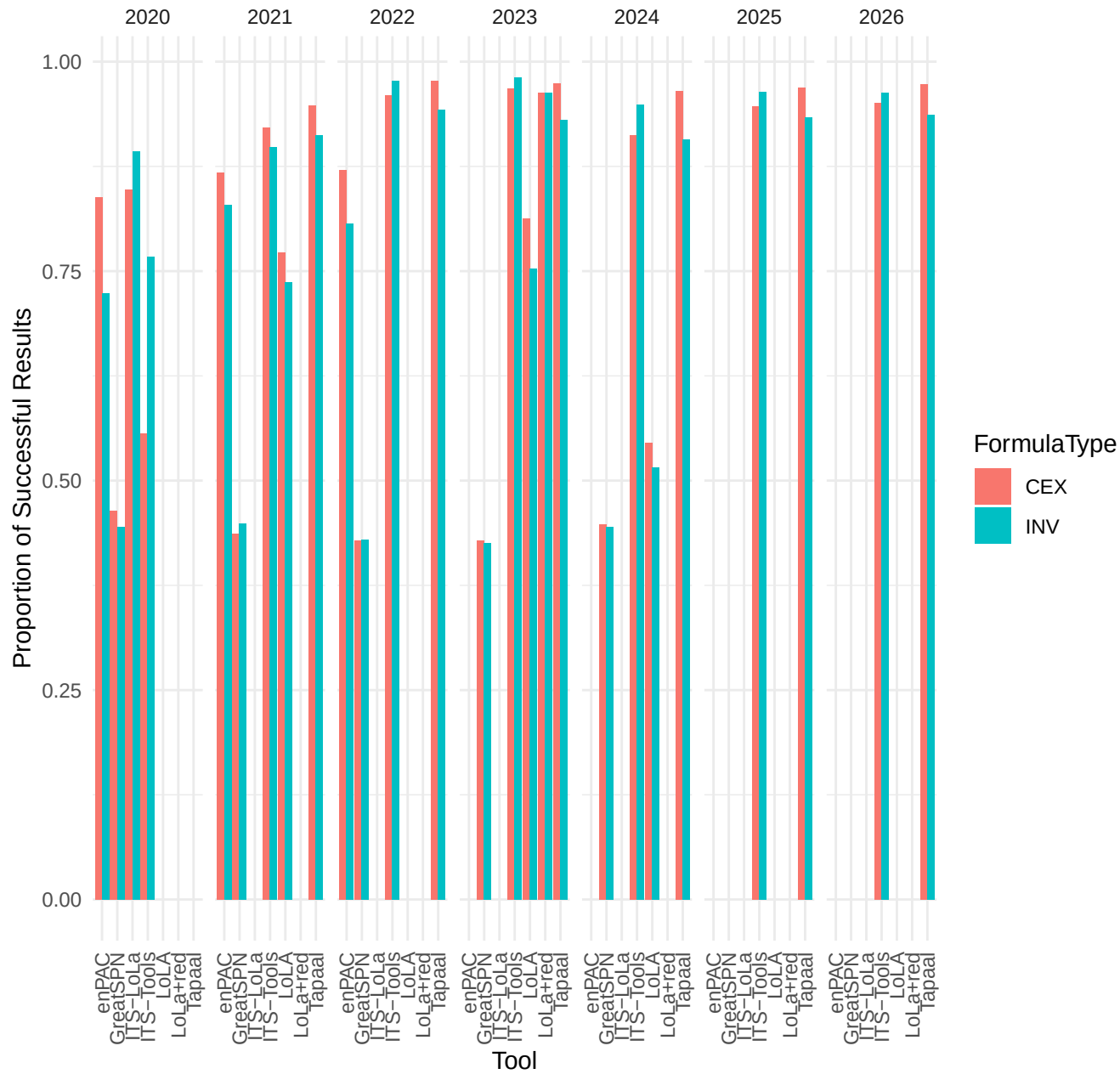
Performance of Main Tools for Itl
