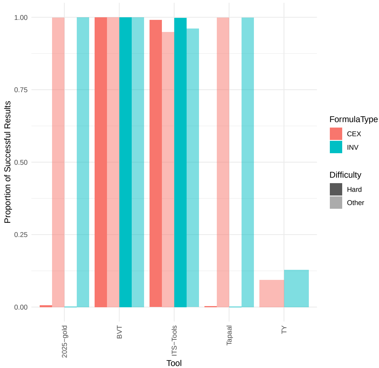
Performance of Main Tools for Itl in 2026
