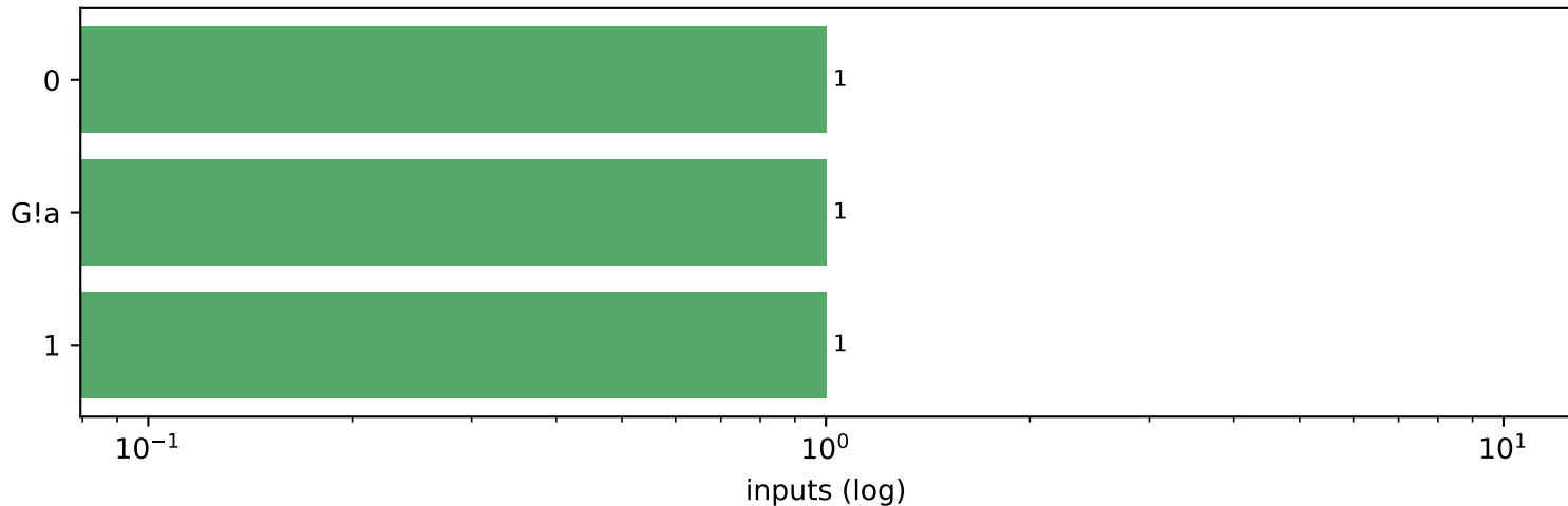
Top 3 reconstructed structures
