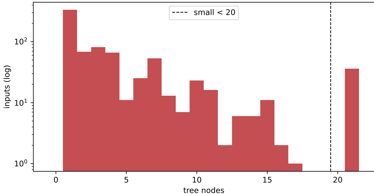
Flattened size (tree nodes); clipped at 21 (36 larger pooled at right)
