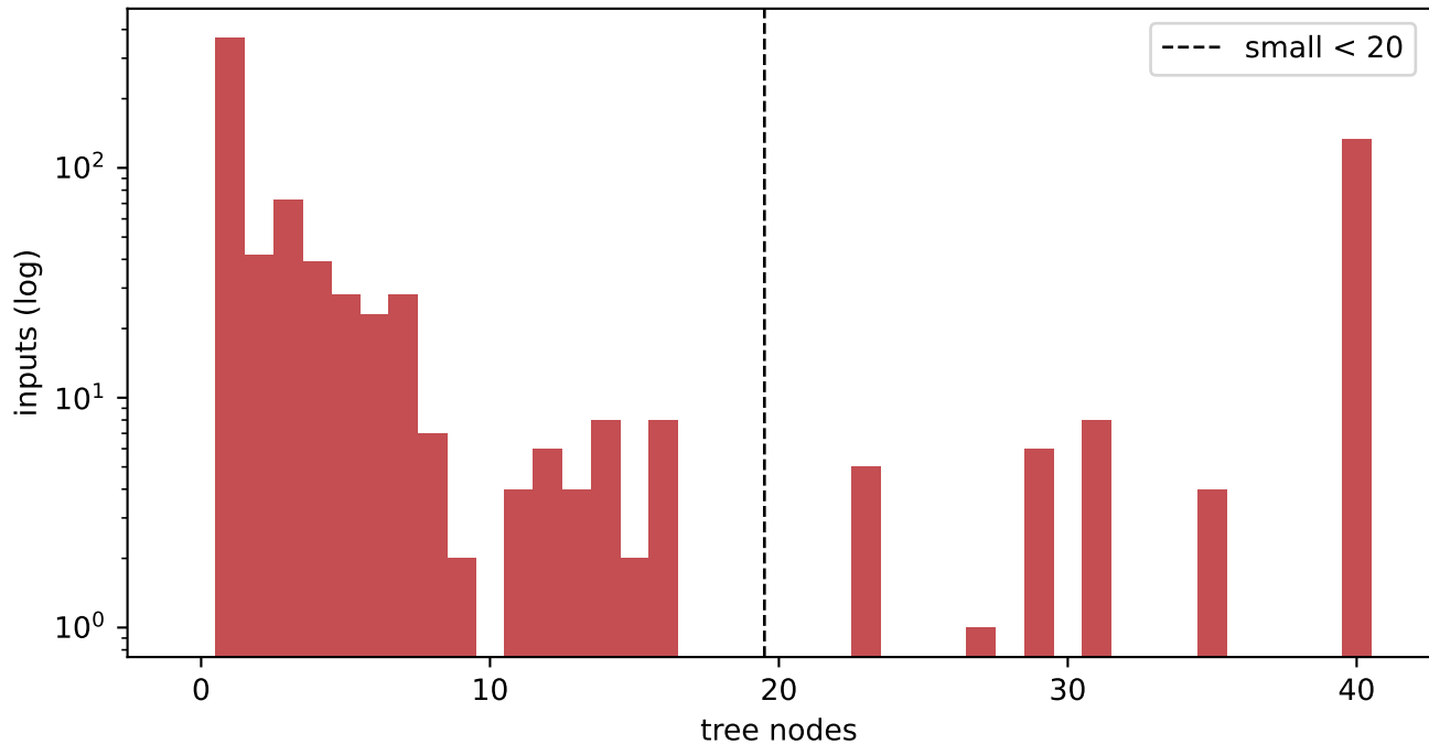
Flattened size (tree nodes); clipped at 40 (134 larger pooled at right)
