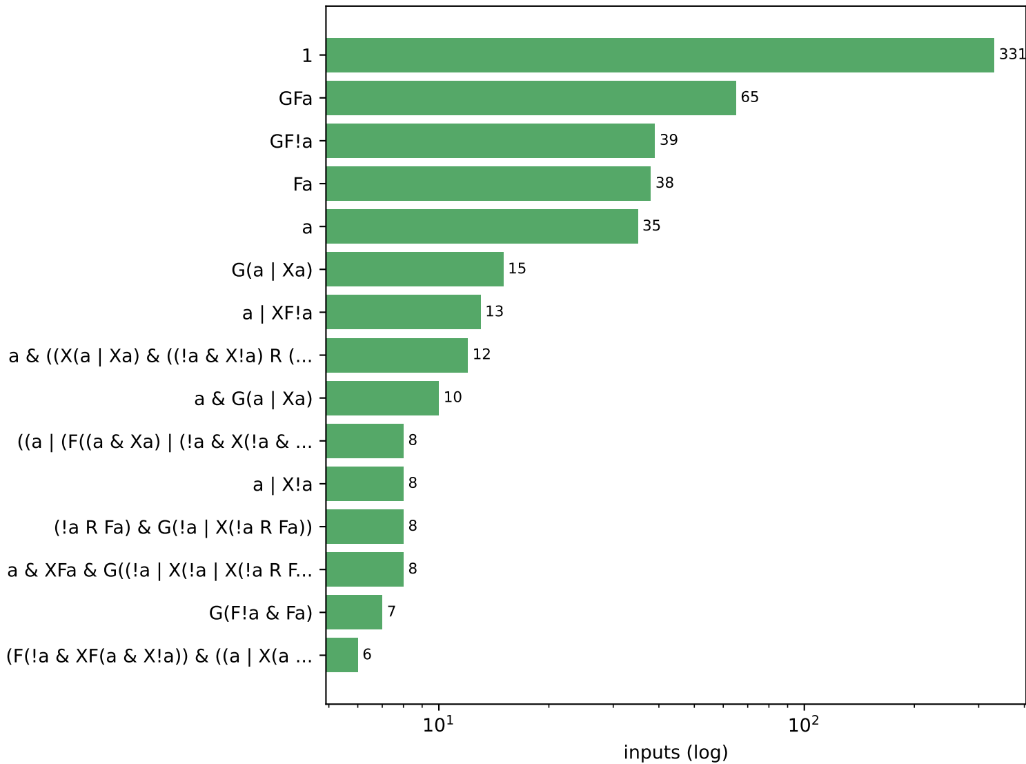
Top 15 reconstructed idioms
