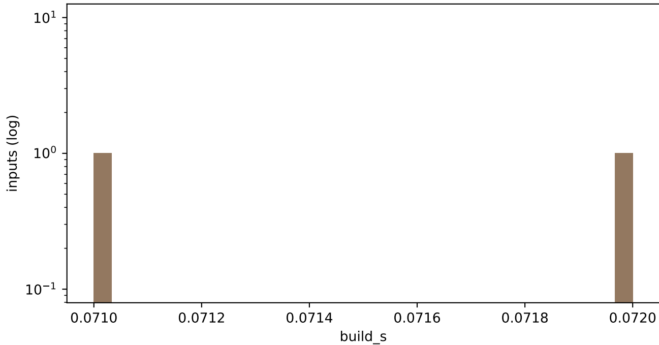
Build-time distribution
