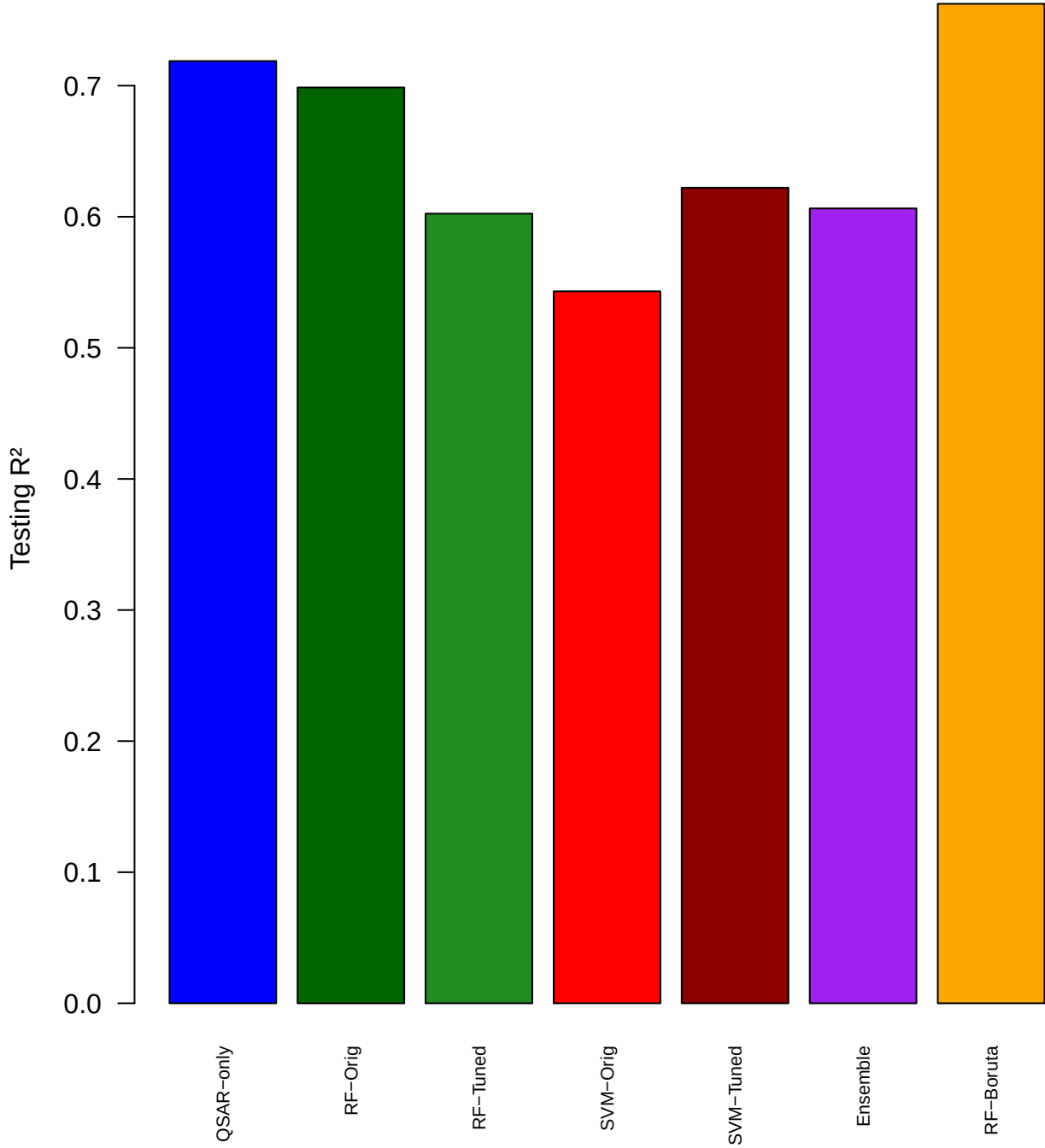
Model Performance Comparison (R 2 )
