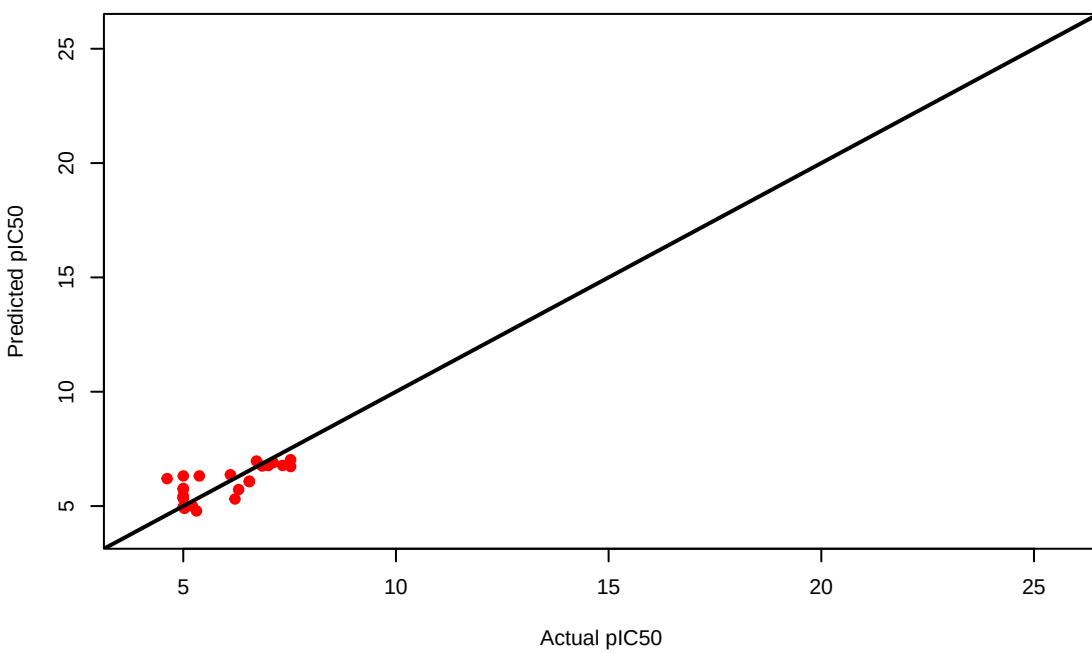
Original SVM ( R^2 = 0.543 )
