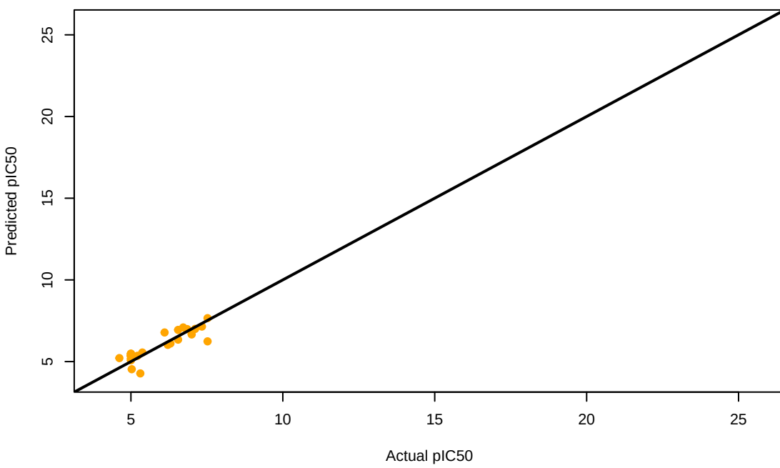
RF Boruta-Selected ( R^2 = 0.762 )
