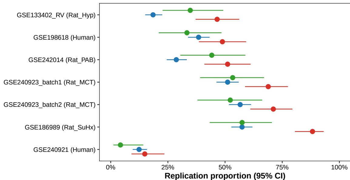
C. Pooled external replication model (7 datasets)
