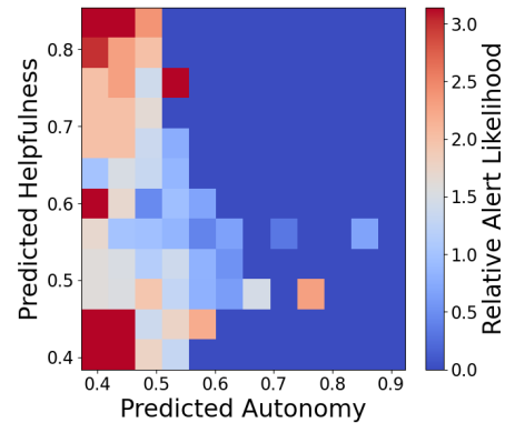
Fig. 3: Visualization of the learned alert policy over the normalised autonomy–helpfulness state space. The space is discretized into a grid, and each cell shows the relative alert likelihood normalized by the overall alert rate. Values greater than one indicate higher-than-average alert frequency. Sparsely populated regions are smoothed using nearest-neighbor interpolation.
