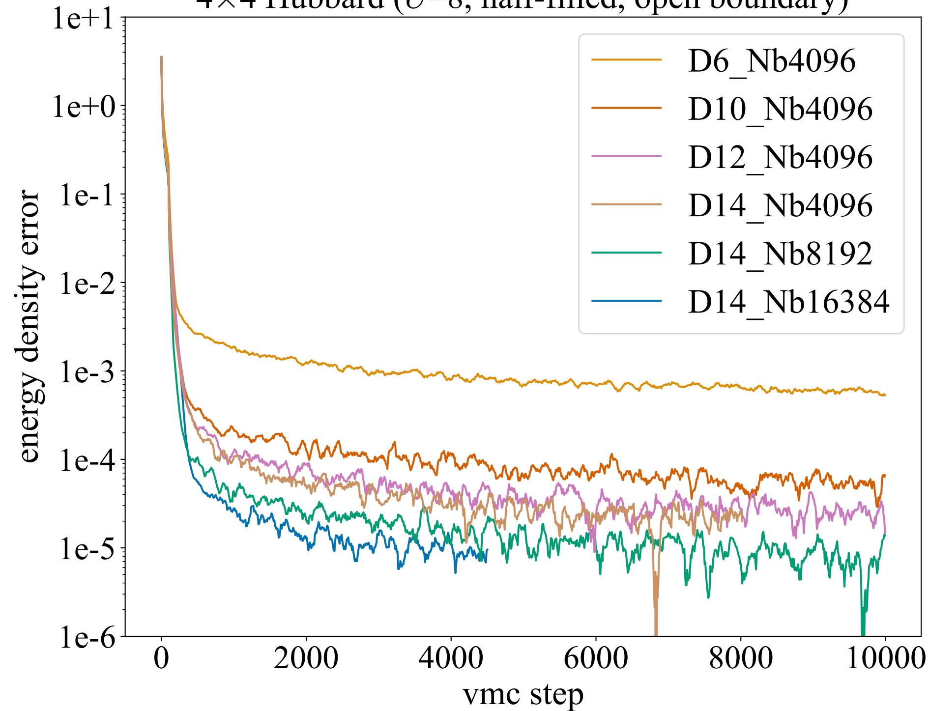
4×4 Hubbard ( U=8 , half-filled, open boundary)
