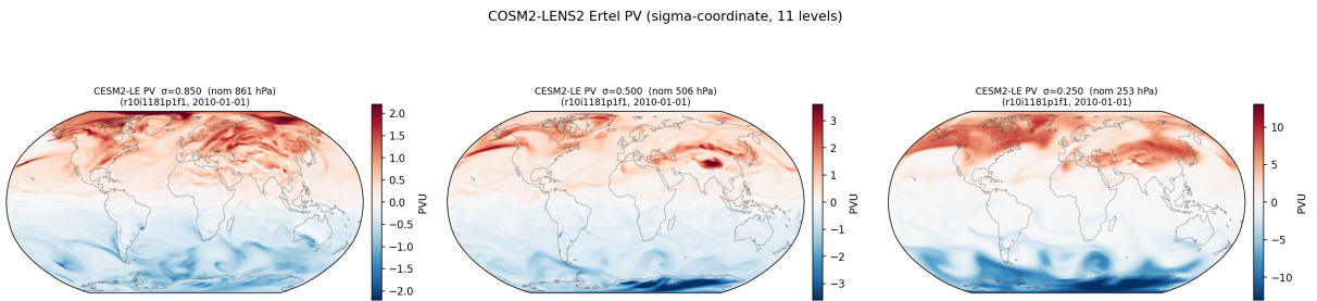
Figure 3: CESM2-LENS2 Ertel PV on 11 sigma levels (2010-01-01). \sigma = 0.85, 0.50, 0.25 .
