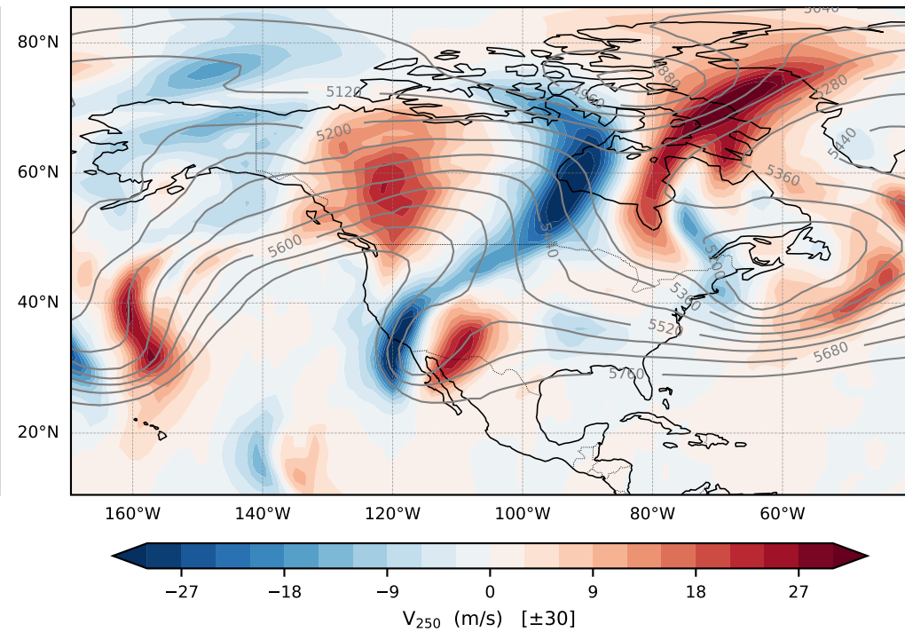
(c) Upper trop. (600-250 hPa)
