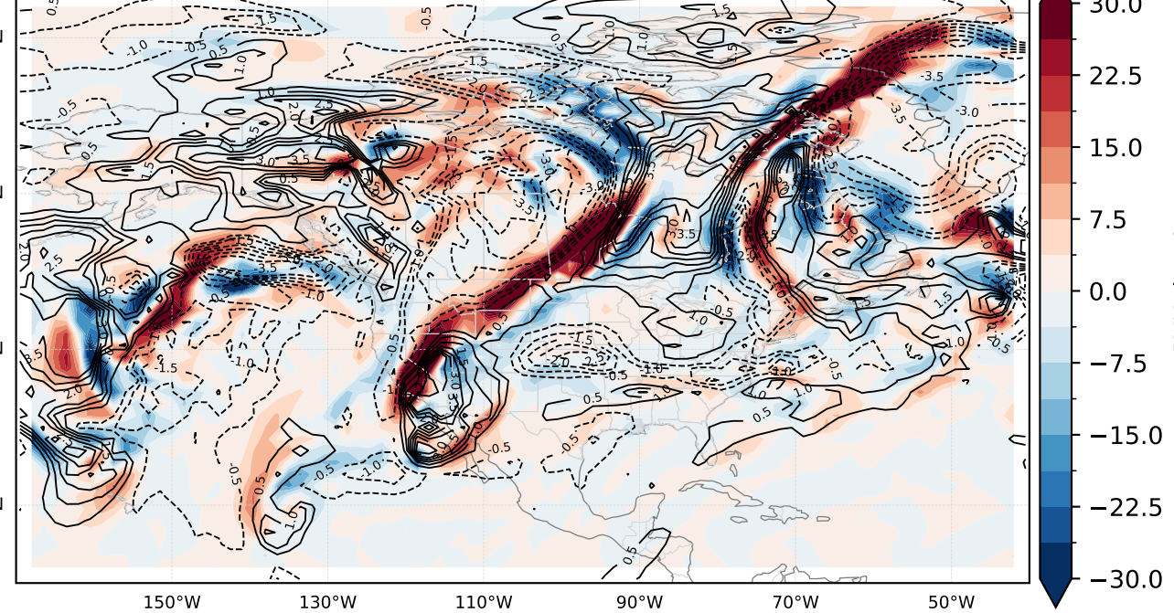
(a) -(\mathbf{u}' \cdot \partial \mathbf{q}' / \partial \mathbf{x} + \mathbf{v}' \cdot \partial \mathbf{q}' / \partial \mathbf{y}) (direct ERA5)
