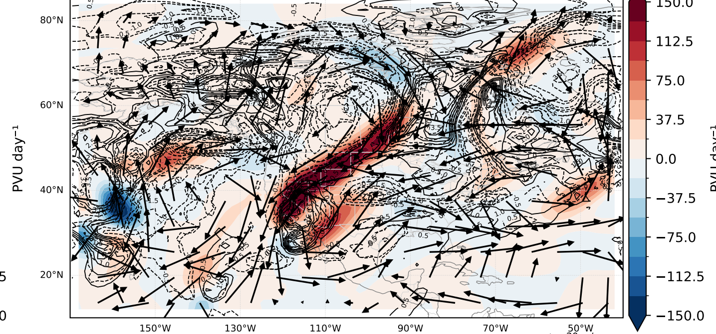
(f) Upper piece: 300-200 hPa
