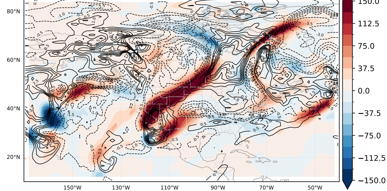
(b) \Sigma pieces (lower + middle + upper)
