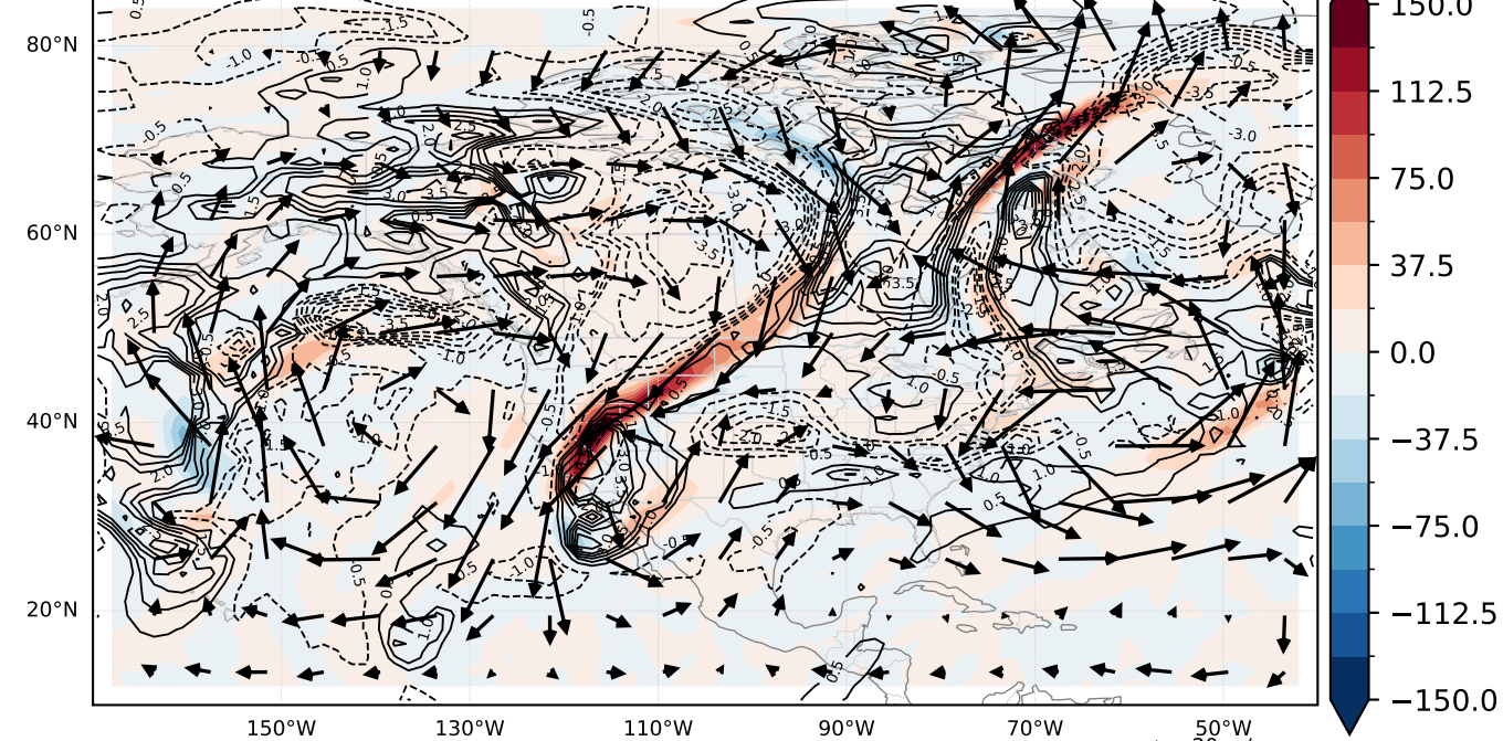
(e) Middle piece: 700-400 hPa
