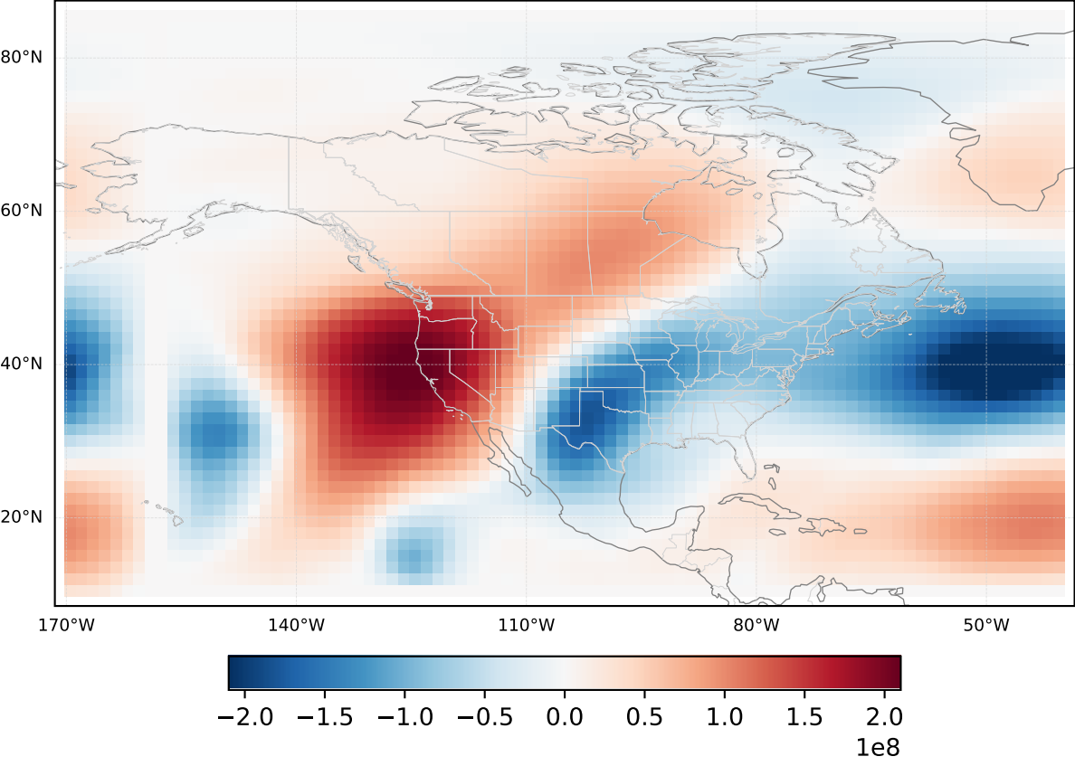
\Sigma pieces vs Total @ 250 hPa
