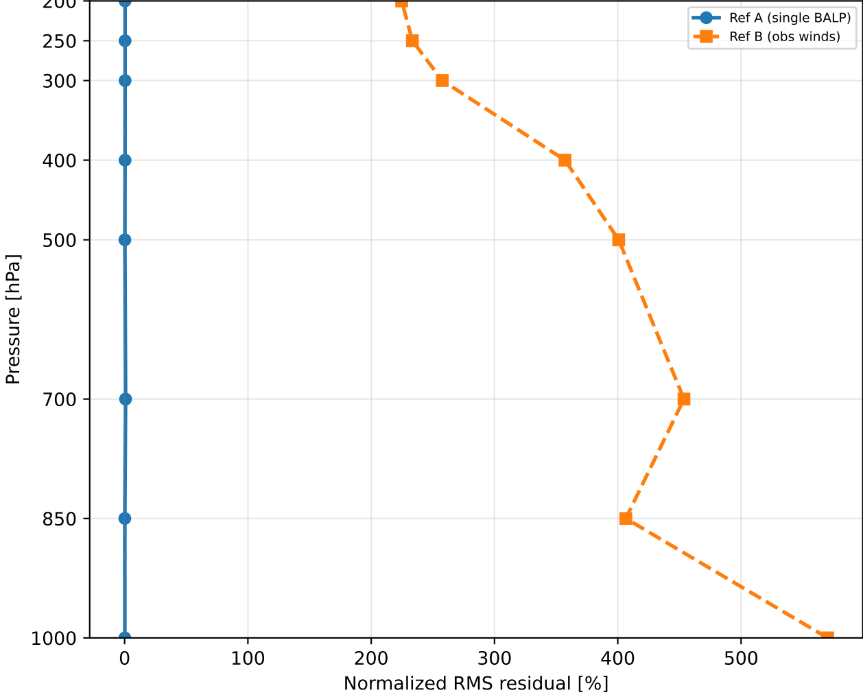
Vertical Profile: nRMS Residual
