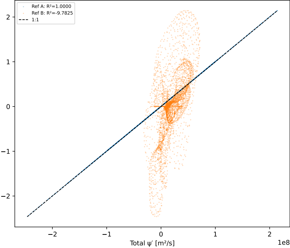
\Sigma pieces vs Total @ 250 hPa
