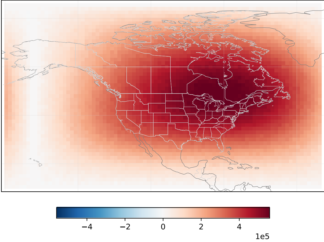
Residual ( \Sigma - \text{Total} )
