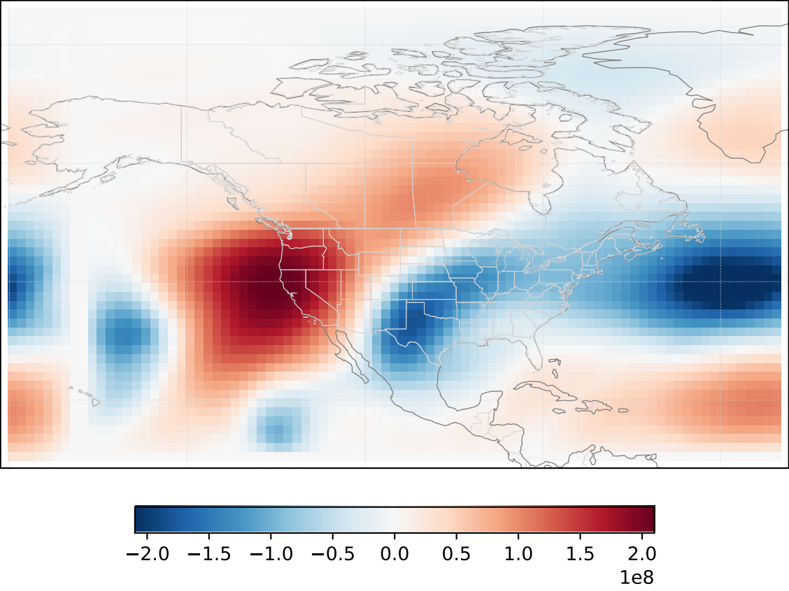
Total \psi' (single BALP)
