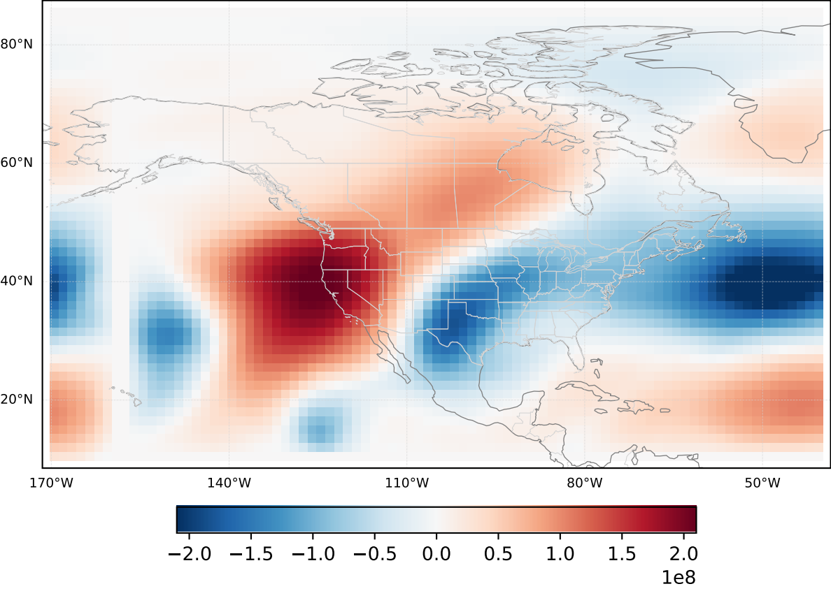
\Sigma pieces \psi' (250 hPa)
