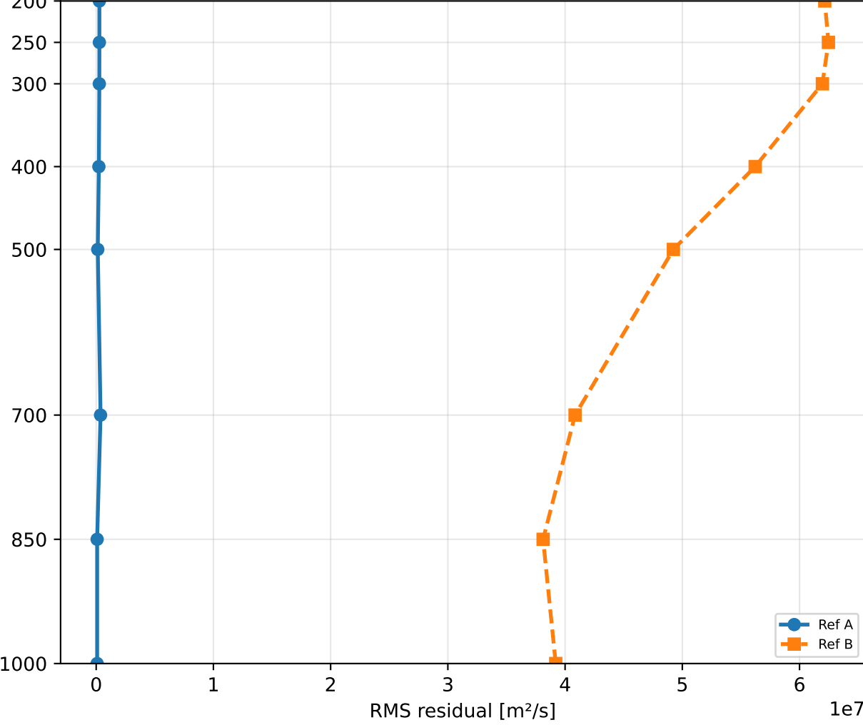
Vertical Profile: RMS Residual
