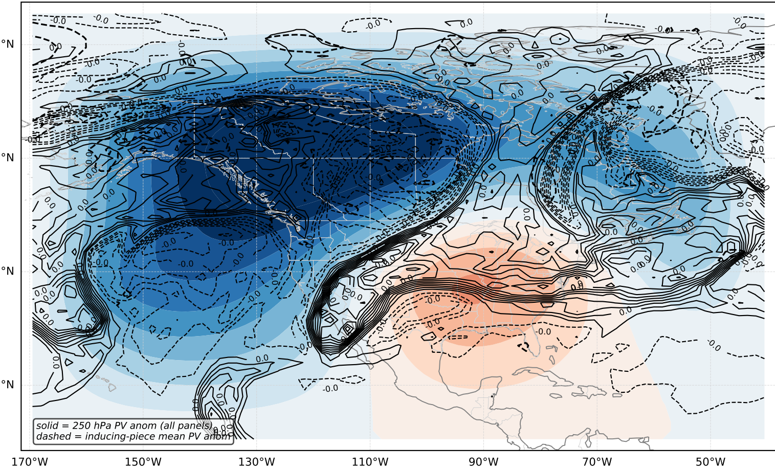
Lower (1000-850 hPa)
