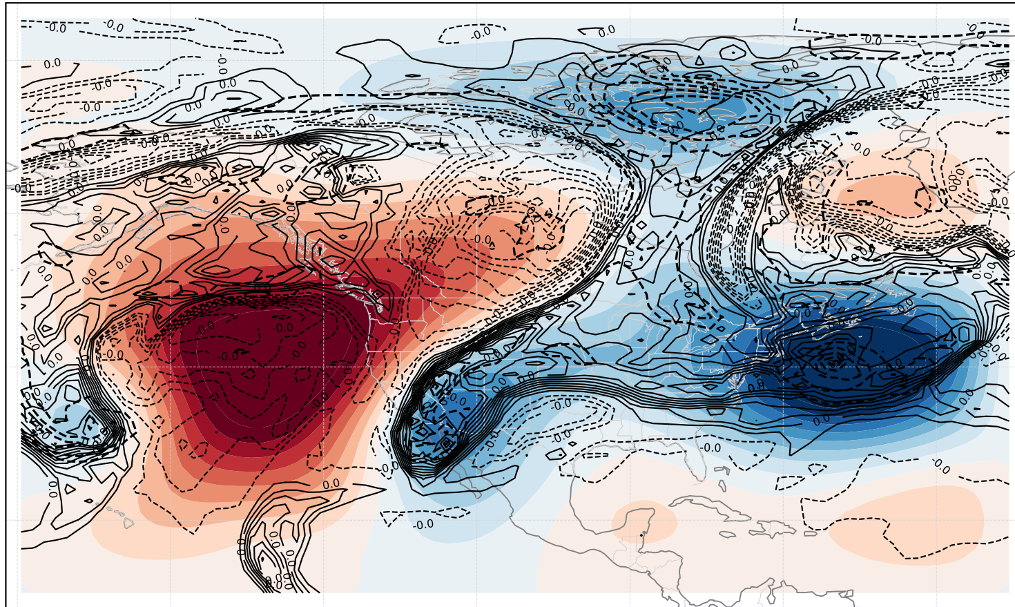
Middle (700-400 hPa)
