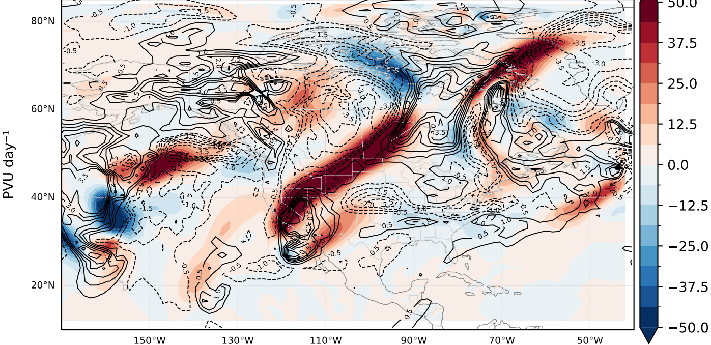
(b) \Sigma pieces (lower + middle + upper)
