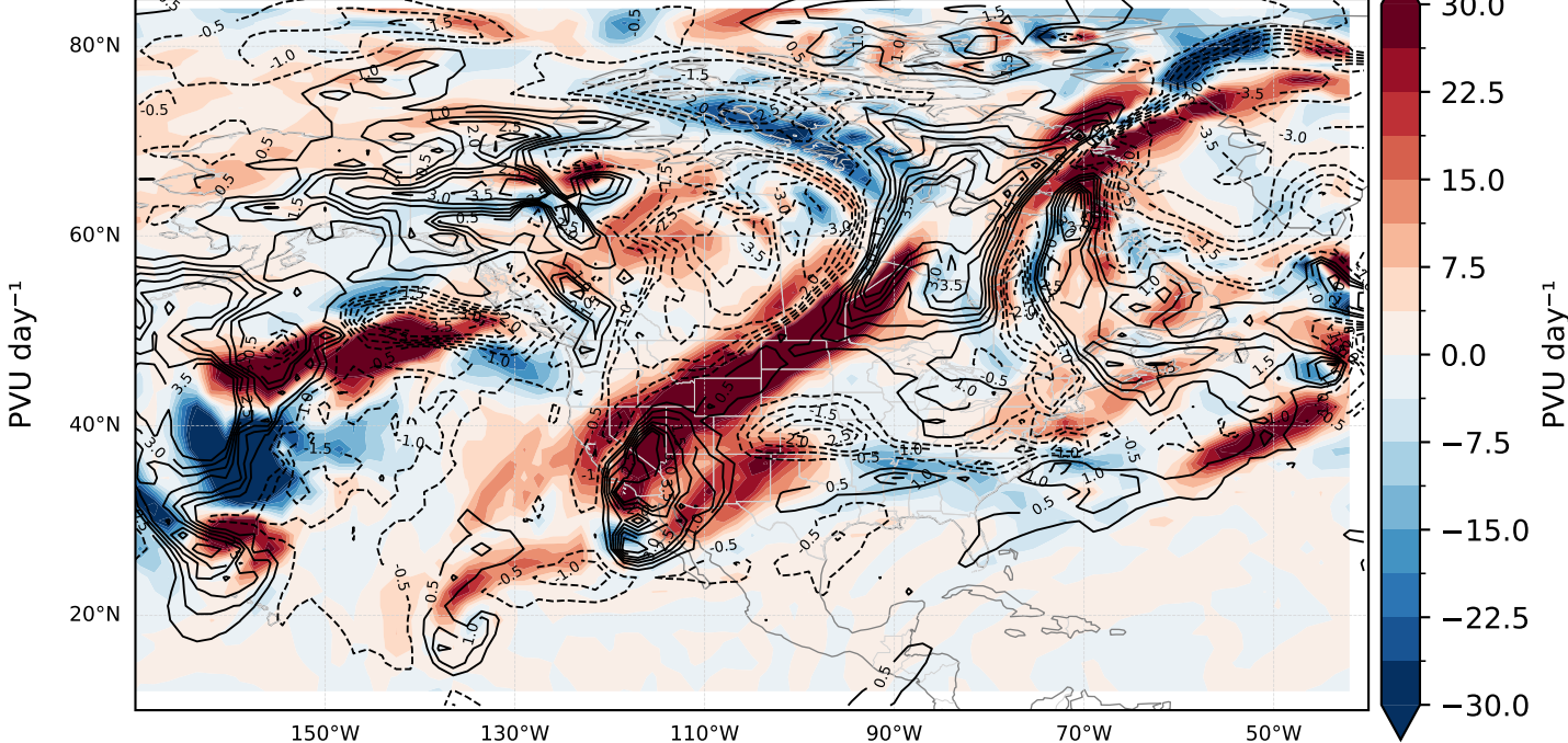
(c) \Sigma pieces - direct (difference)
