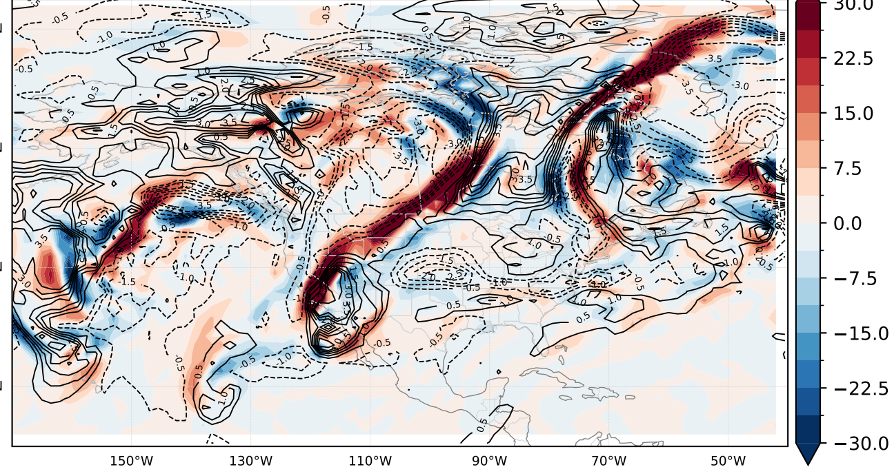
(a) -(u' \cdot \partial q' / \partial x + v' \cdot \partial q' / \partial y) (direct ERA5)
