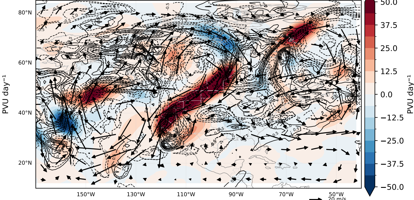
(f) Upper piece: 300-200 hPa
