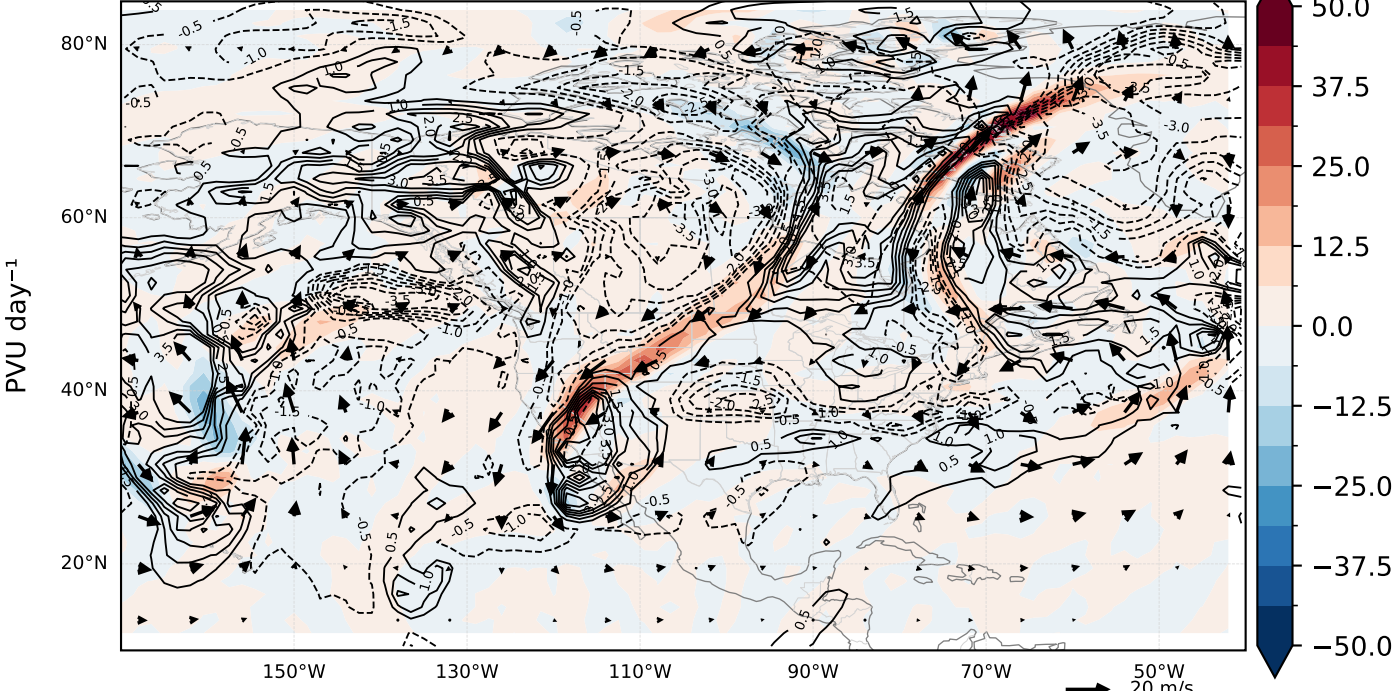
(e) Middle piece: 700-400 hPa
