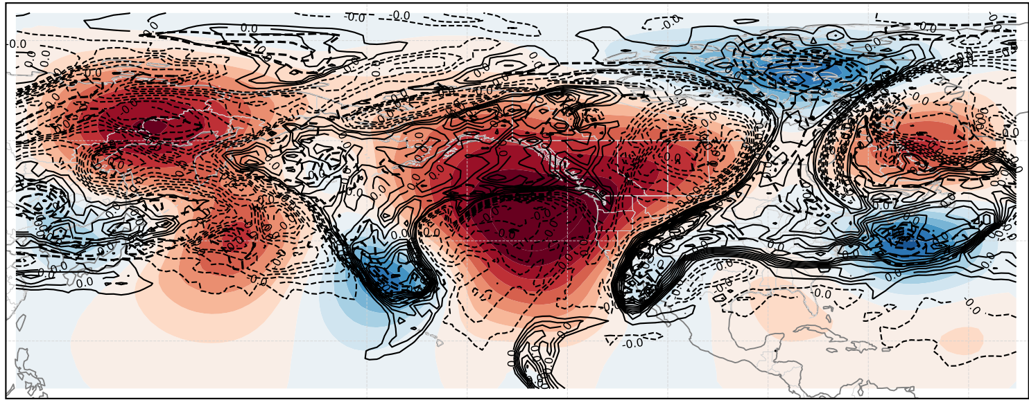
Middle (700-400 hPa)
