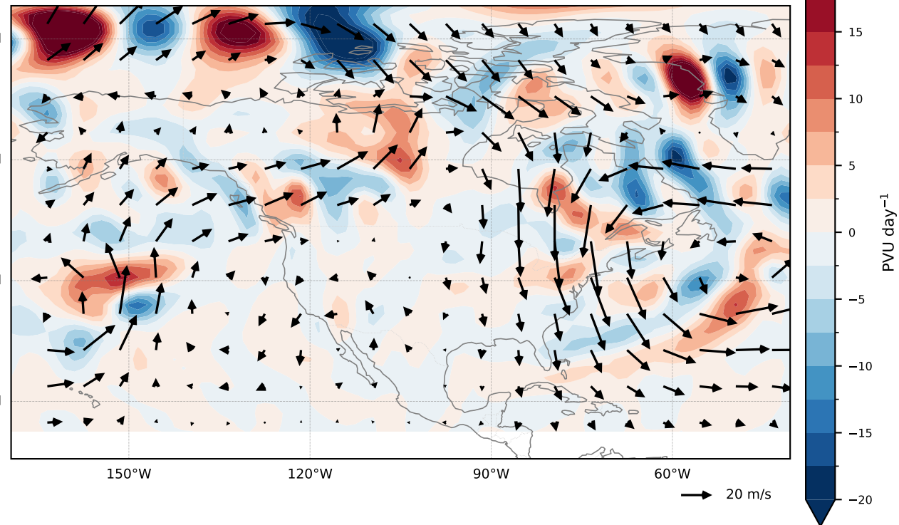
(c) Upper (300/250 hPa) ( |\max|=20 PVU/day)
