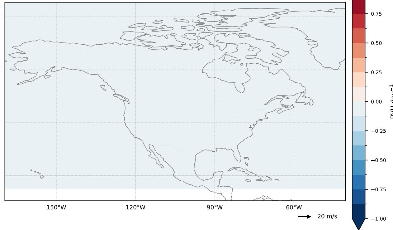
(a) Lower (850/700 hPa) ( |\max|=1 PVU/day)
