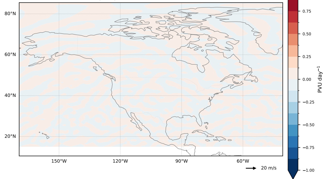
(b) Middle (500/400 hPa) ( |\text{max}|=1 PVU/day)
