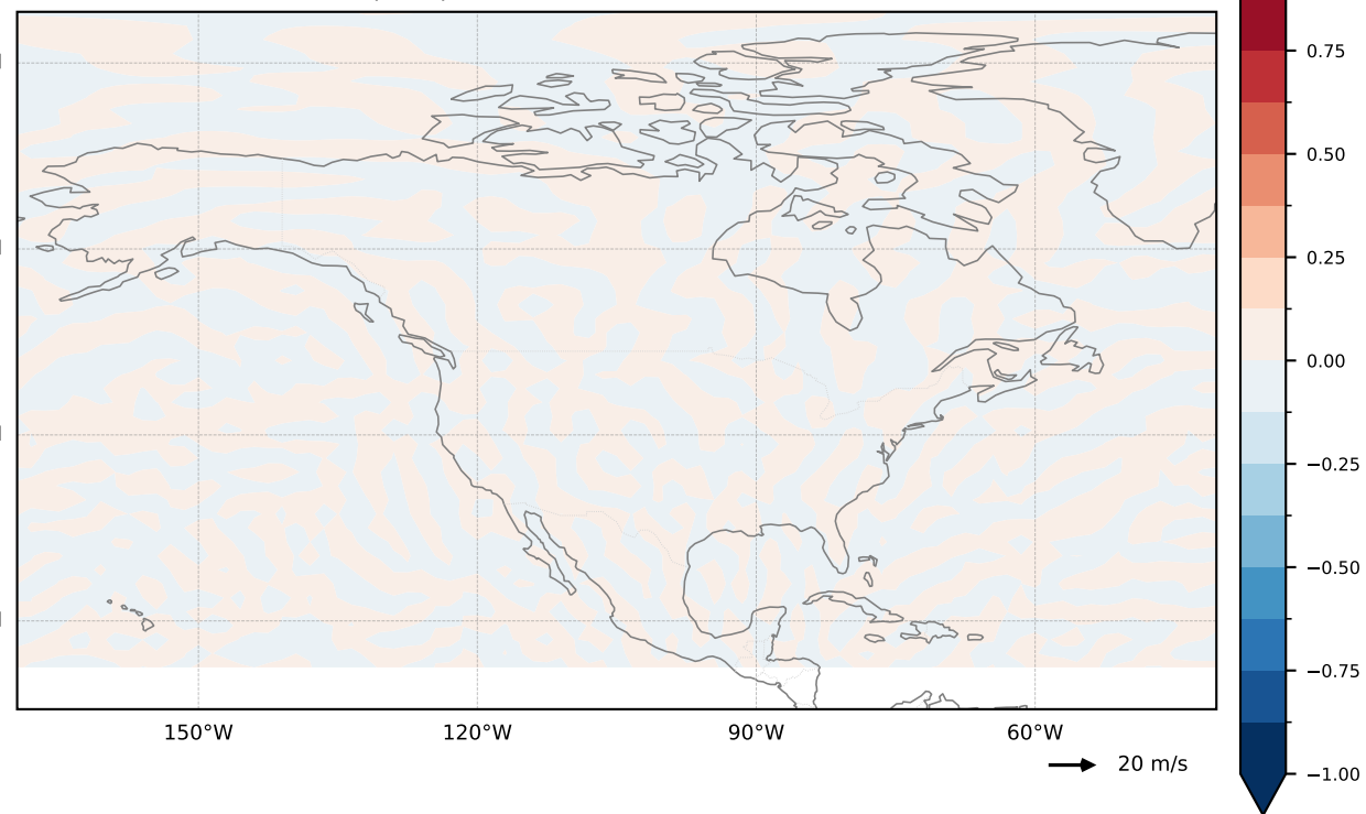
(a) Lower (850/700 hPa) ( |\text{max}|=1 PVU/day)
