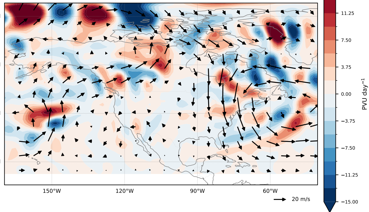
(c) Upper (300/250 hPa) ( |\text{max}|=15 PVU/day)
