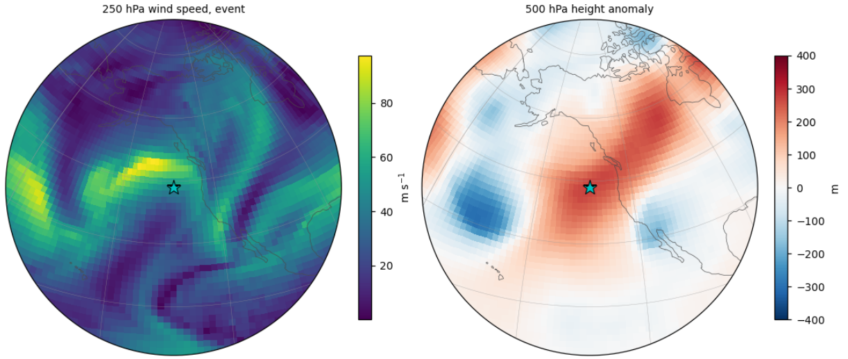
Figure 1: The event: wind speed at 250 hPa, and the 500 hPa height anomaly against the climatology. The difference between the two states is what is decomposed: anomalous potential vorticity in the interior, anomalous potential temperature on the top and bottom boundaries.
