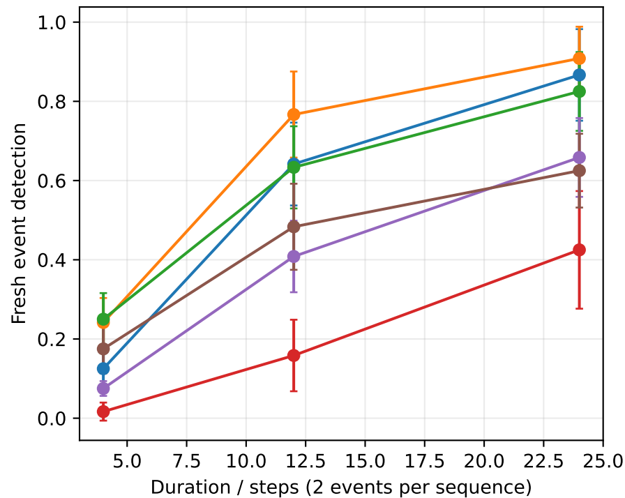
New synthetic validation; fixed event starts; same nominal q99; error bars: seed SD
