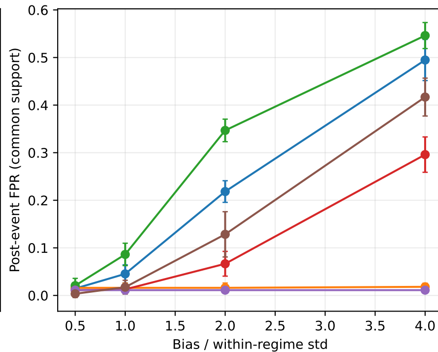
Synthetic validation; five-seed SD; same nominal q99, not matched realized FPR
