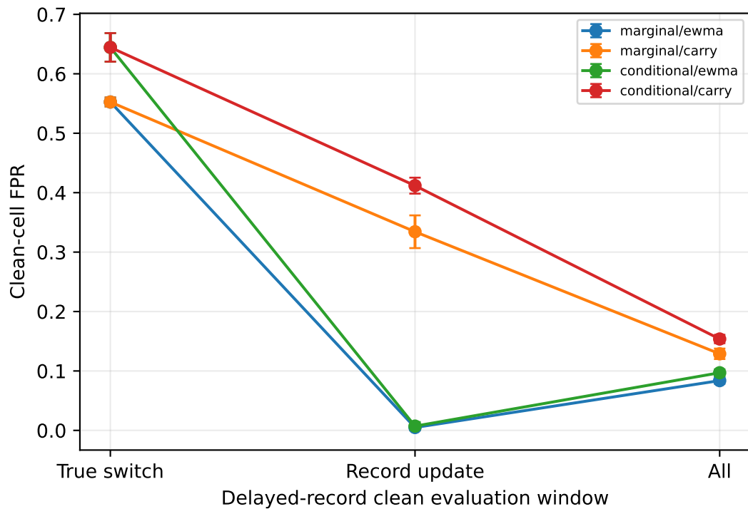
Synthetic paired reset ablation; fixed thresholds; error bars: seed SD
