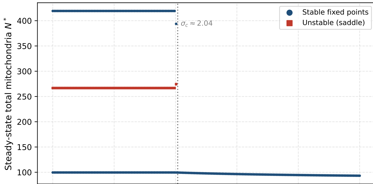
Bifurcation Diagram: Mitochondrial Network (saddle-node with cooperative ROS feedback, Hill n = 2 )
