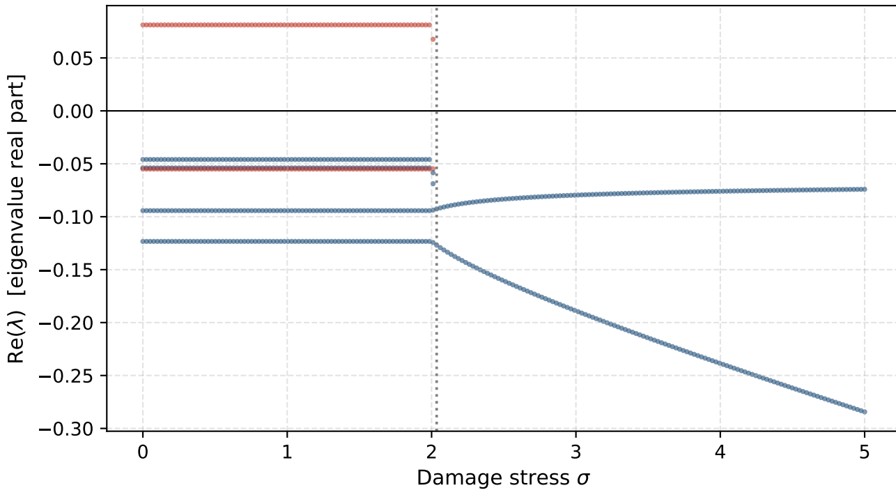
Jacobian eigenvalues vs. stress
