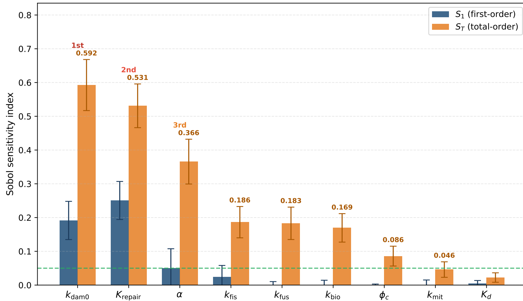
Global Sensitivity of \sigma_c to Model Parameters (Sobol indices, saddle-node bifurcation of mitochondrial network)
