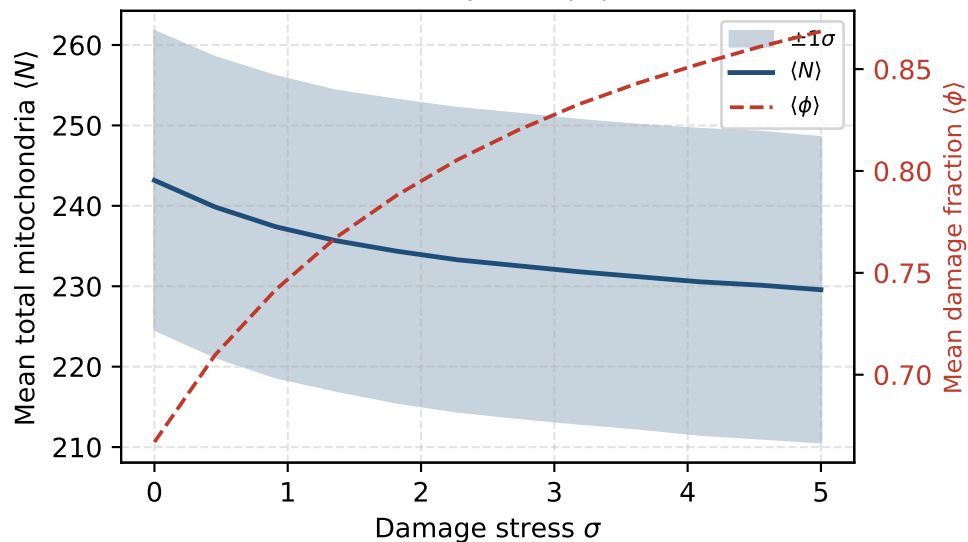
(a) Mean steady-state population
