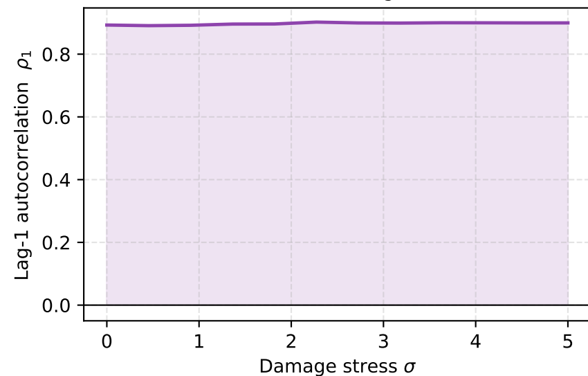
(c) Critical slowing down
