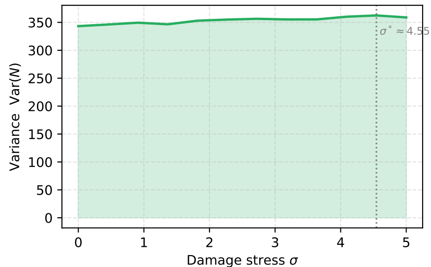
(b) Critical fluctuations
