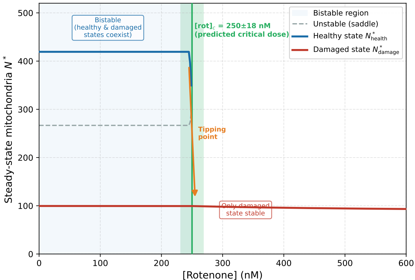
Prediction 1 — Rotenone Dose-Response Curve (Saddle-node bifurcation of mitochondrial network, Hill n = 2 ROS feedback)
