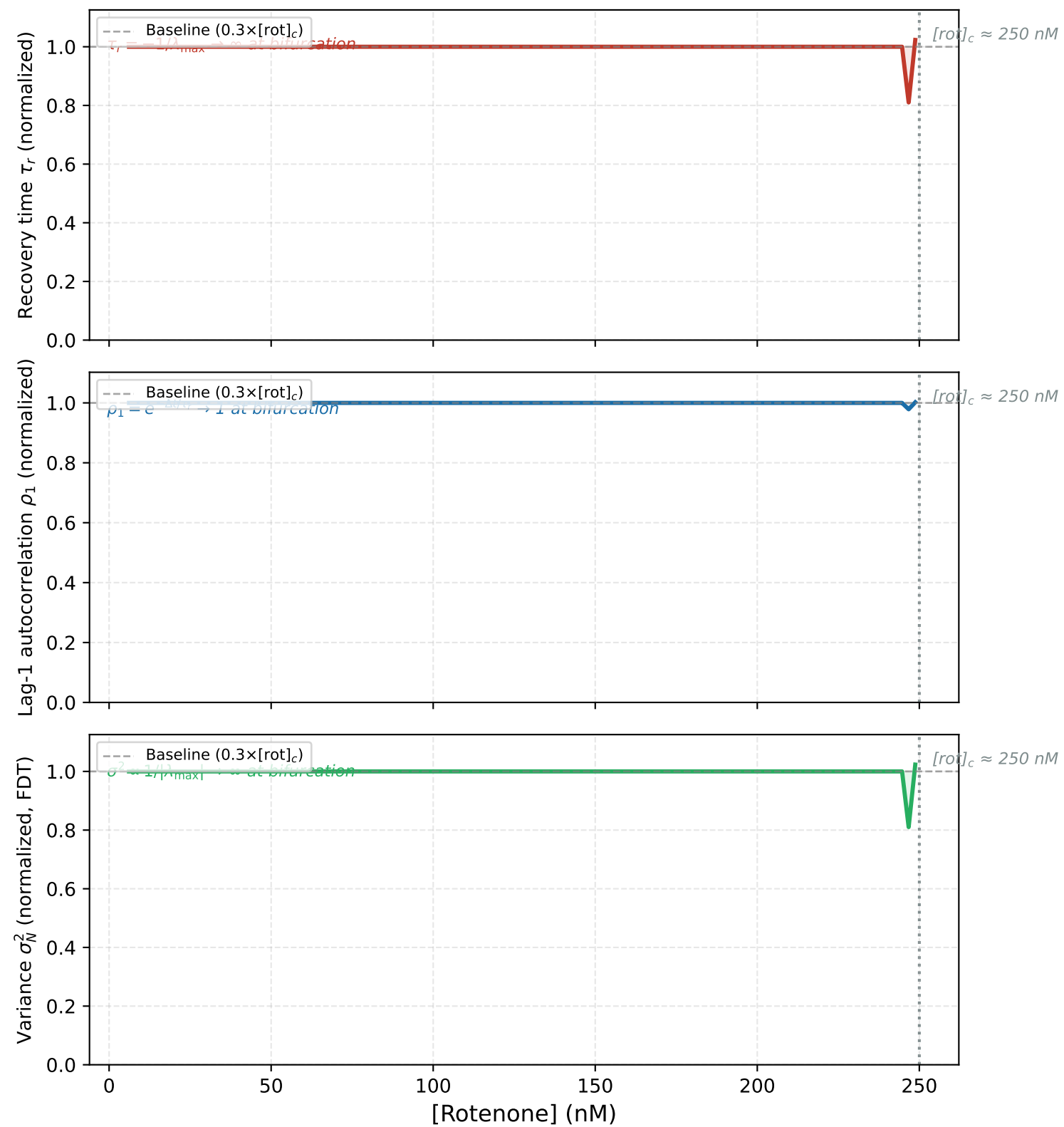
Prediction 2 — Early Warning Signal Metrics vs [Rotenone] (Theoretical from ODE Jacobian \lambda_{\max} , normalized to baseline)
