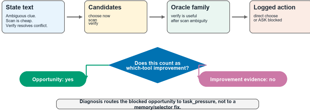
Figure 4: Case-step visualization. A step can count as a tool-choice opportunity while still failing the locked memory comparison because the selected action does not realize the oracle verify family.
