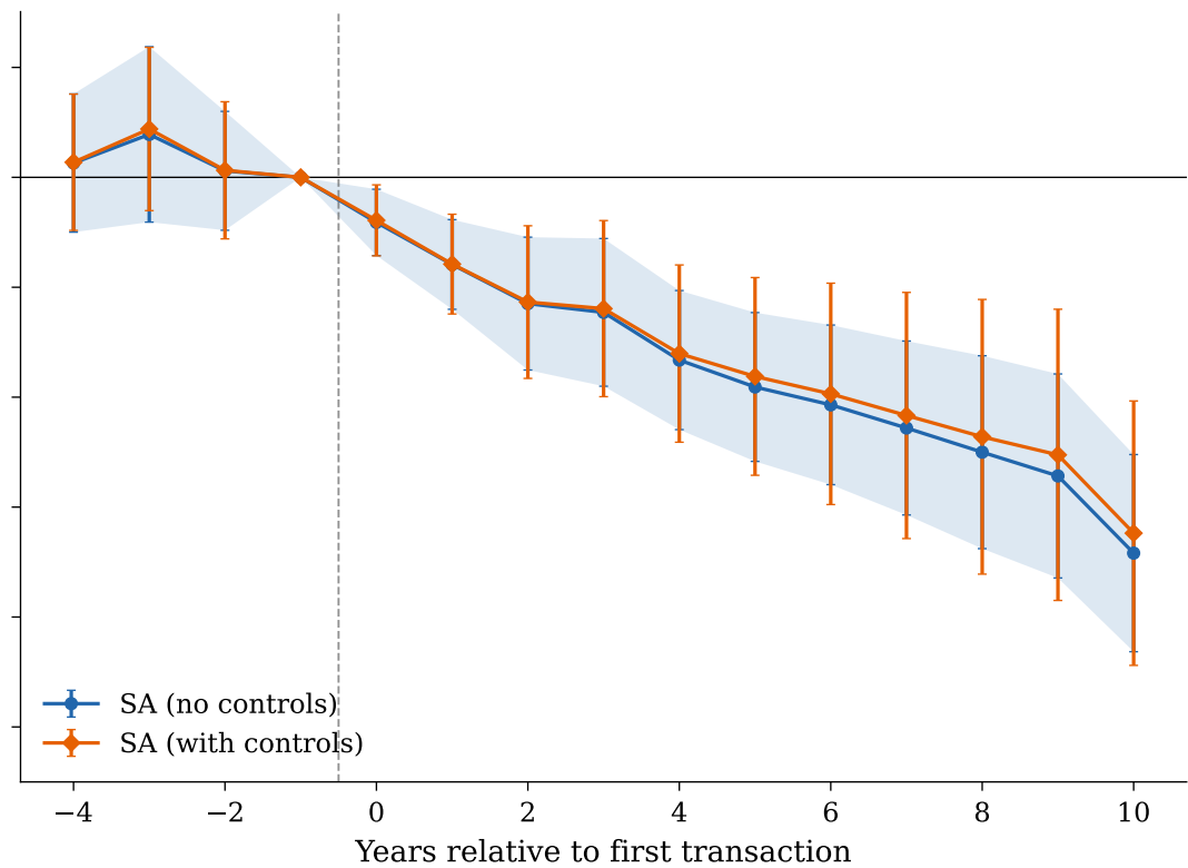
(b) Sun-Abraham
