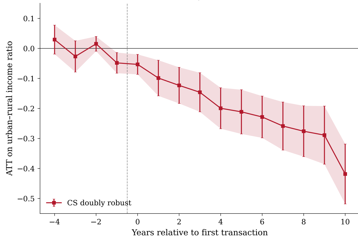
(a) Callaway-Sant'Anna
