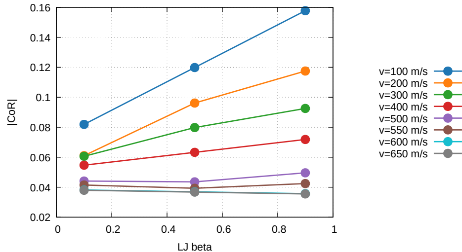
Effect of LJ beta on coefficient of restitution
