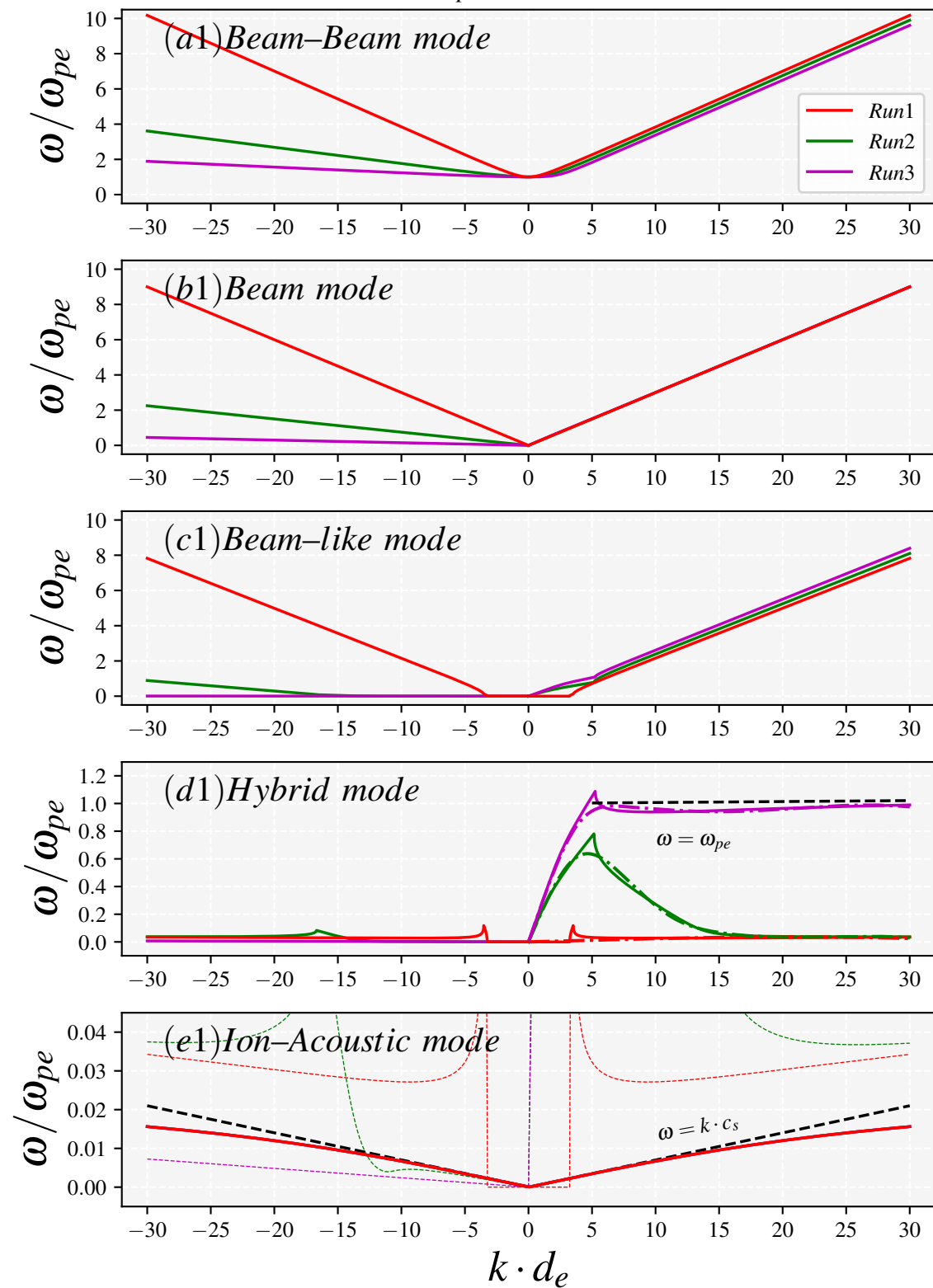
Dispersion Relation
