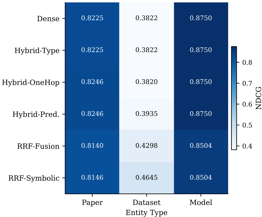
Retrieval Method
