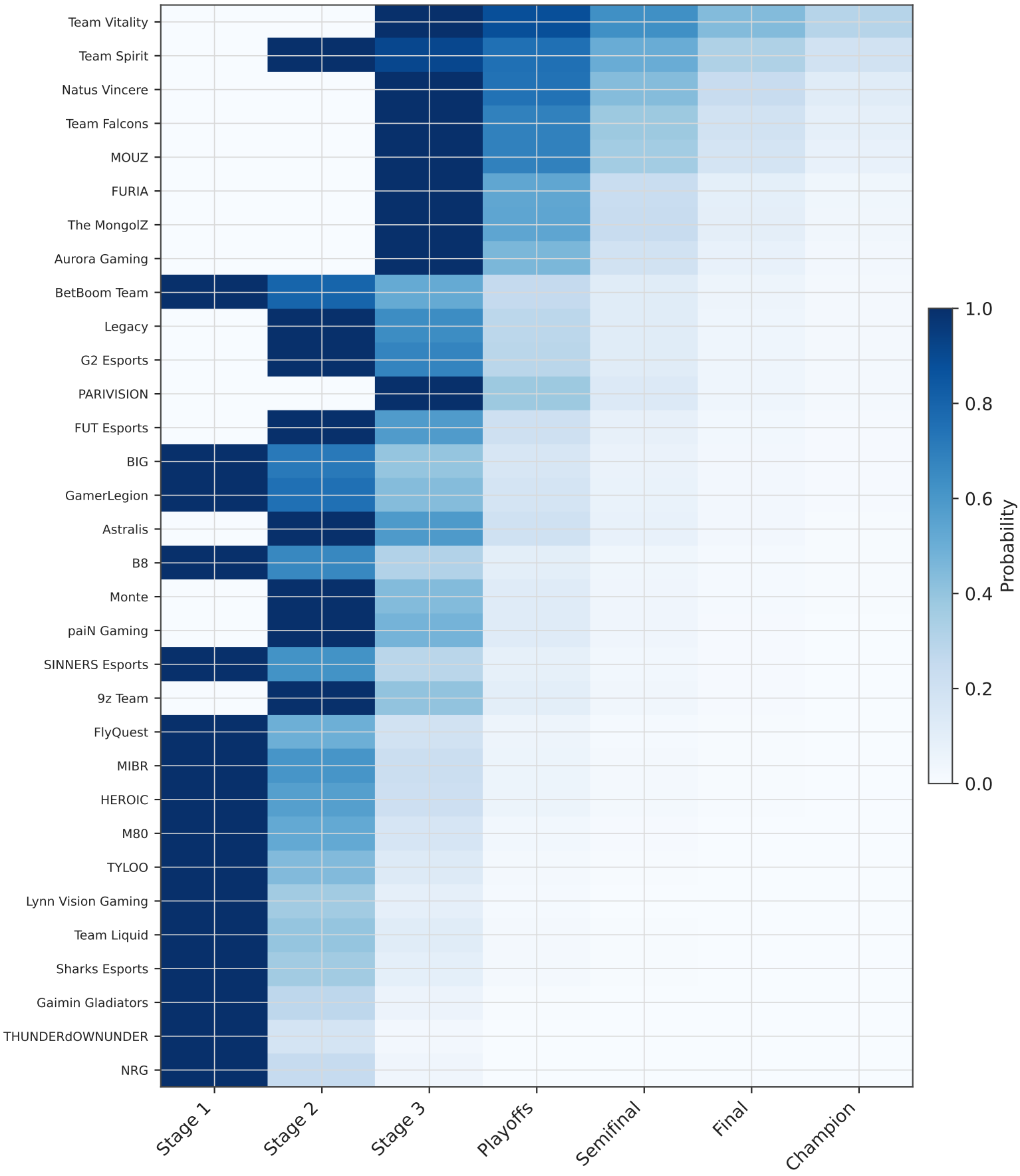
Stage Progression Probability Matrix
