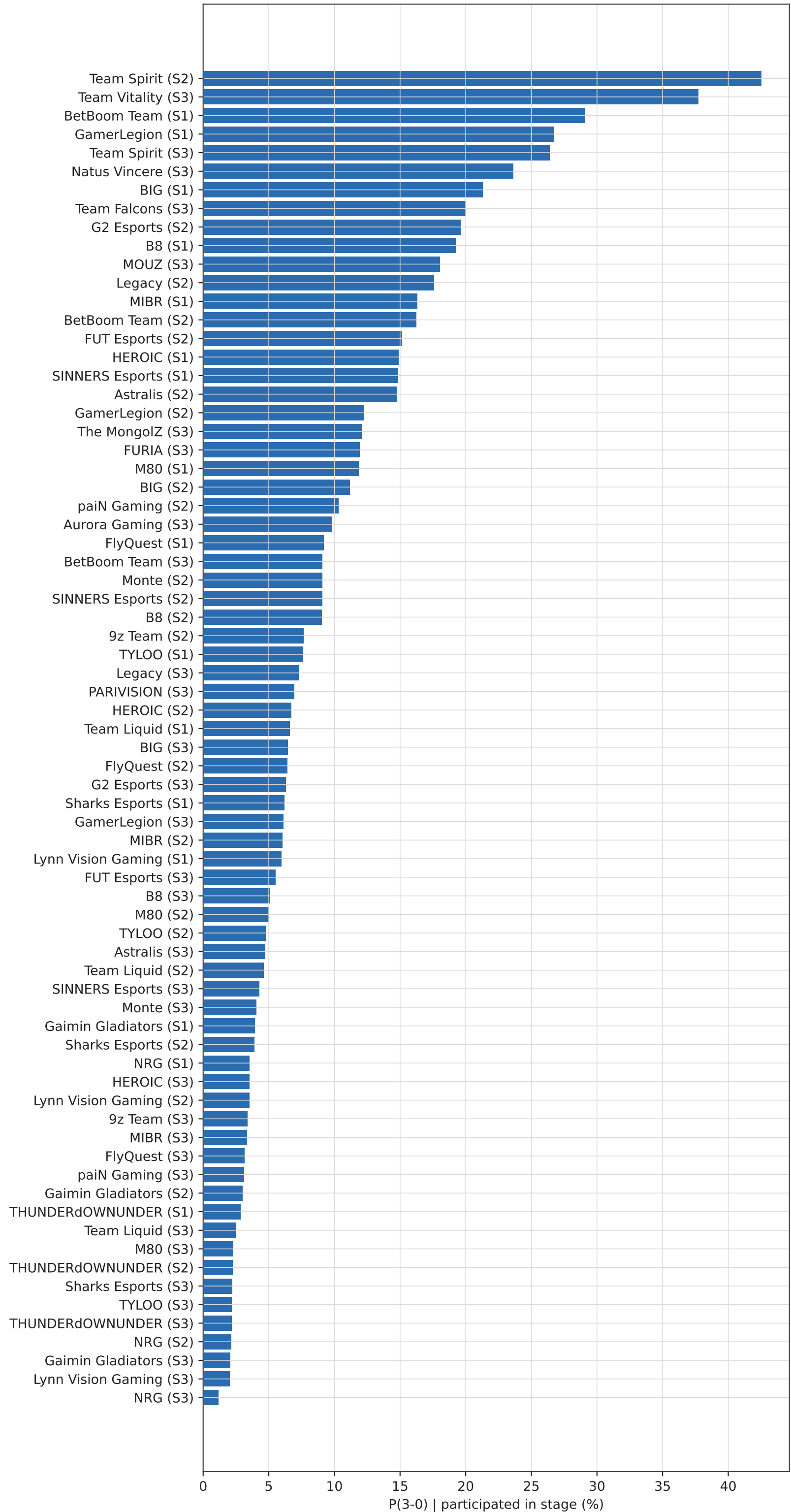
3-0 Sweep Probability, by Swiss-Stage Participant
