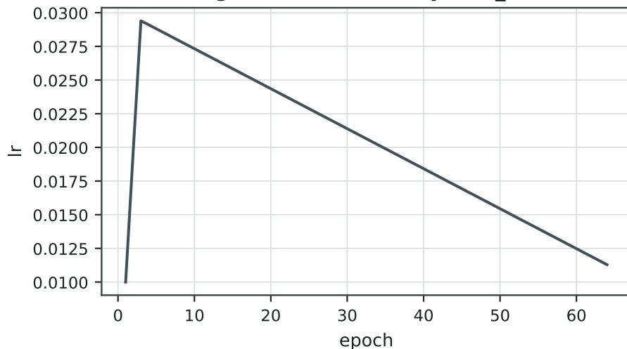
Learning rate (linear decay, cos_lr=false)
