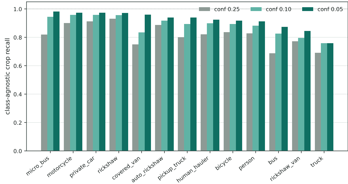
Stage 1 per-class crop recall at three operating points (test split)
