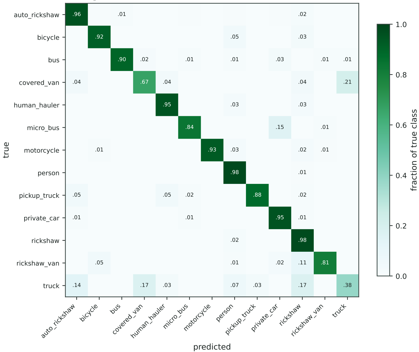
Stage 2 v1 — row-normalised confusion matrix (test)
