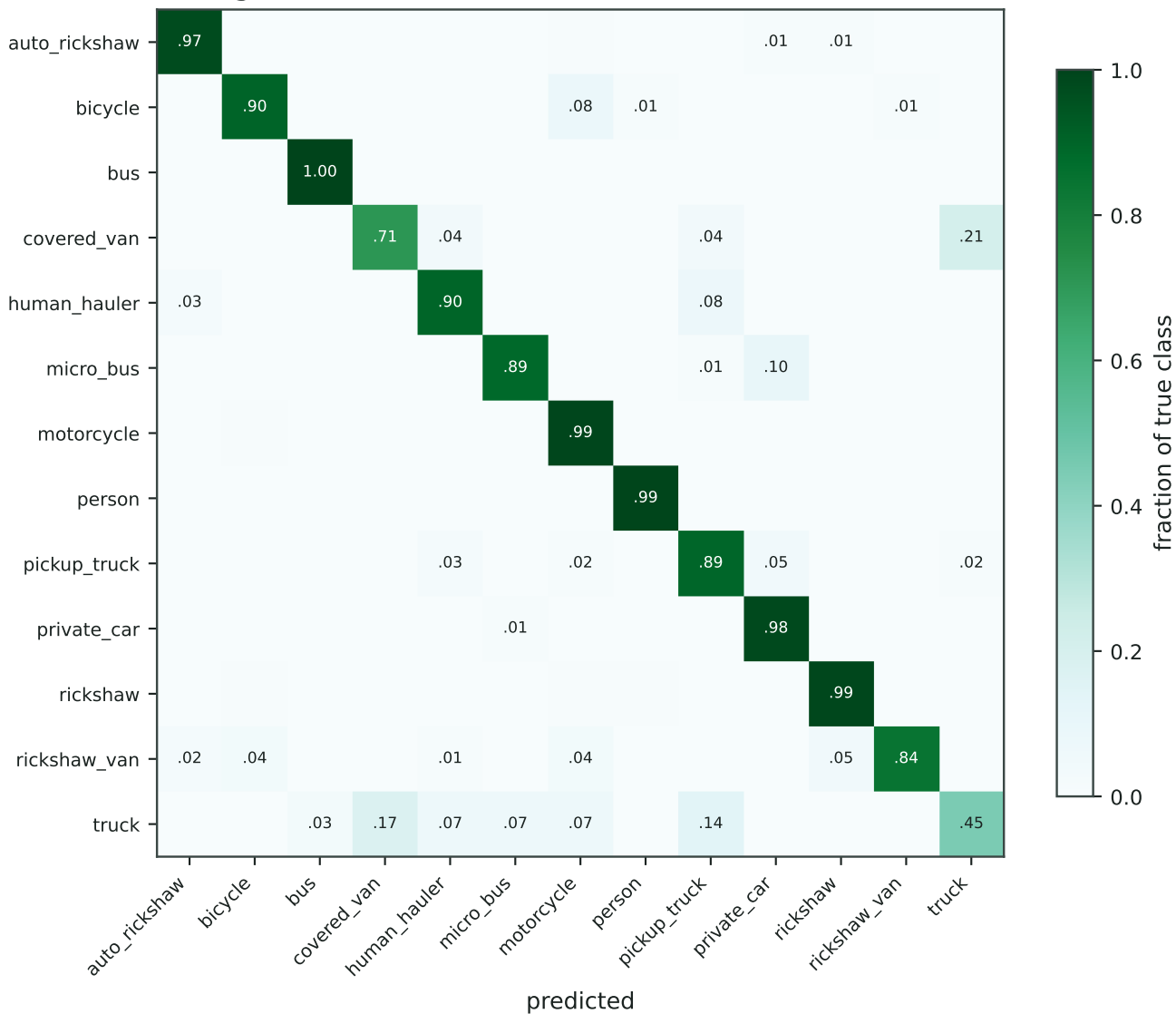
Stage 2 v2 — row-normalised confusion matrix (test)
