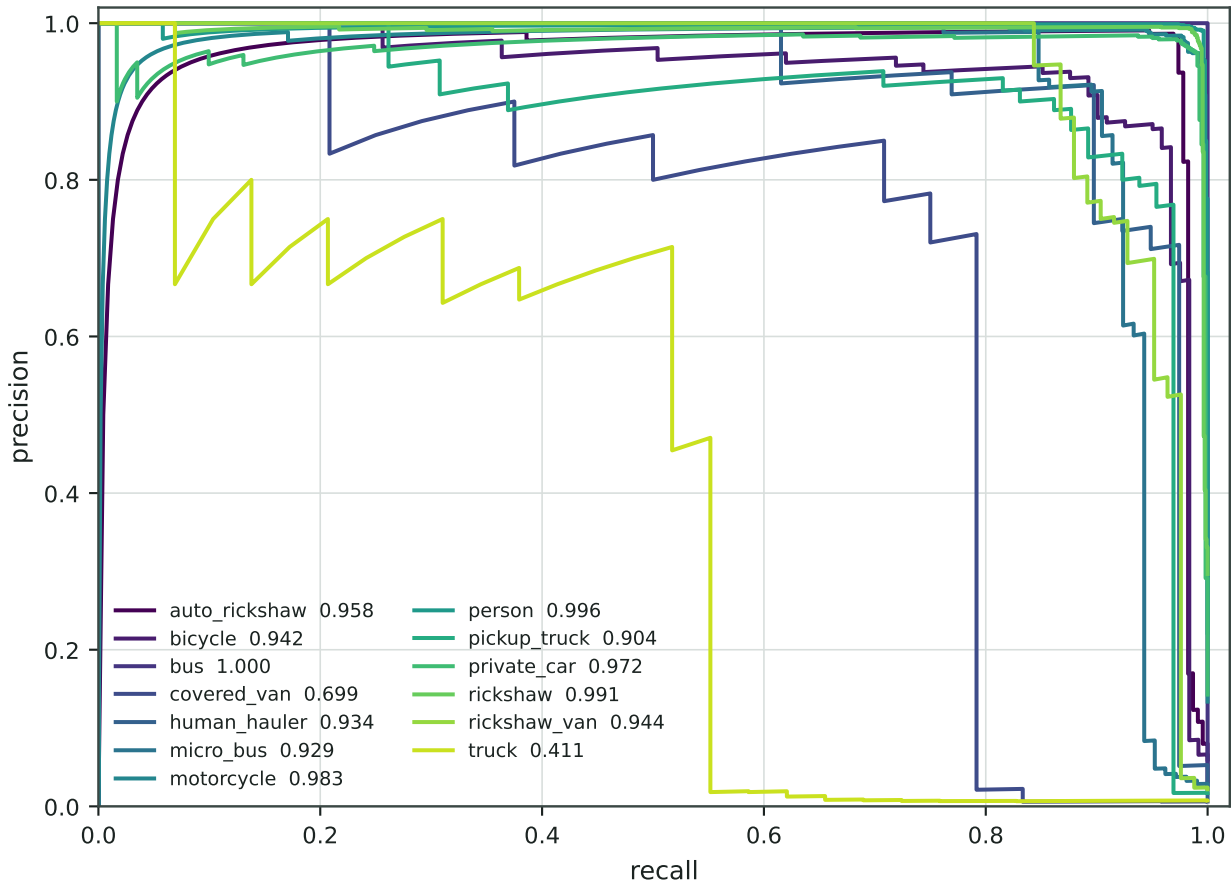
Stage 2 per-class precision-recall (test, GT crops) — macro AP 0.897
