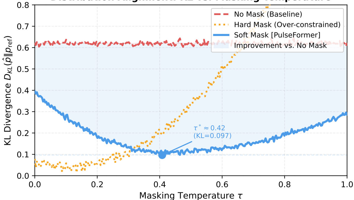
Distribution Alignment: KL vs. Masking Temperature
