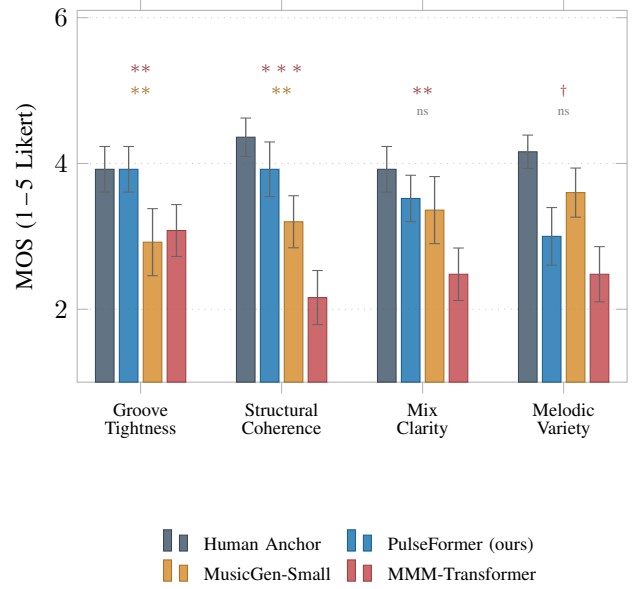
Fig. 5. MOS results ( N = 25 , 95 % CI; Wilcoxon vs. PulseFormer). Stars above bars: sig. vs. MG / MMM-Trans : *** p < 0.001 ; ** p < 0.01 ; ^{\dagger}p < 0.10 ; ns. PF \approx Human Anchor (GT, p = 0.93 ); dominates SC ( p < 0.001 , d > 1.9 ).
