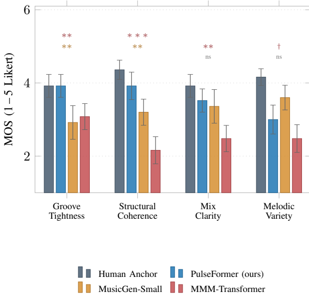
Fig. 5. MOS results ( N = 25 , 95% CI; Wilcoxon vs. PulseFormer). Stars above bars: sig. vs. MGen / MMM-Trans : *** p < 0.001 ; ** p < 0.01 ; † p < 0.10 ; ns. PF \approx Human Anchor (GT, p = 0.93 ); dominates SC ( p < 0.001 , d > 1.9 ).
