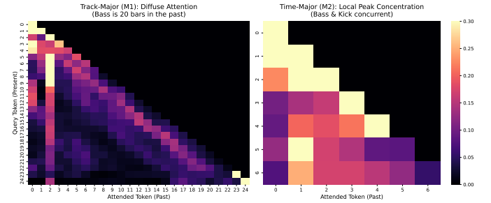
Fig. 4. Extracted generative self-attention matrices (final standard layer). Left (M1): The Track-Major topology forces the model into a diffuse gradient, failing to structurally synchronize Kick boundaries. Right (M2): The Time-Major topology mathematically compels a sharp local attention peak, eliminating physical layout uncertainty.
