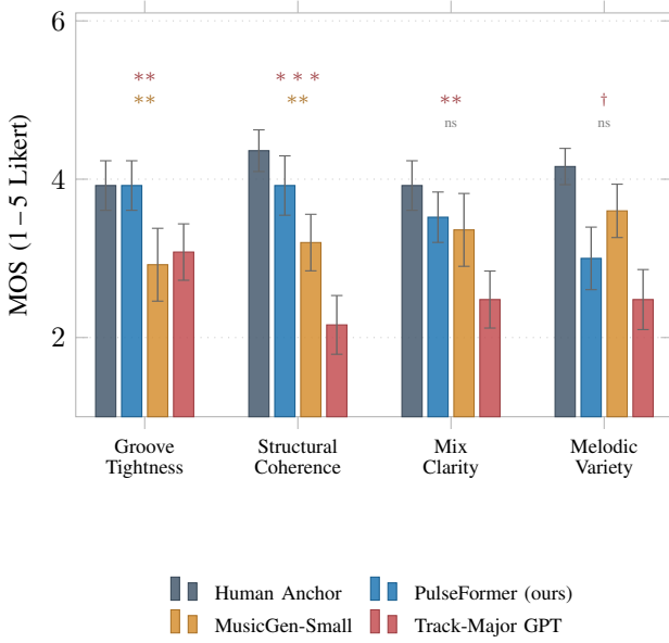
Fig. 4. MOS results ( N = 25 , 95 % CI; Wilcoxon vs. PulseFormer). Stars above bars: sig. vs. MGen / TM-GPT : *** p < 0.001 ; ** p < 0.01 ; † p < 0.10 ; ns. PF \approx Human Anchor (GT, p = 0.93 ); dominates SC ( p < 0.001 , d > 1.9 ).
