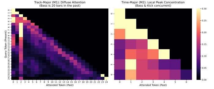
Fig. 6: Extracted generative self-attention matrices (final layer). Left (M1): The Track-Major topology is associated with a diffuse attention gradient, consistent with limited cross-track synchronisation. Right (M2): The Time-Major topology produces a concentrated local attention peak, consistent with the substantially reduced \Delta_{sync} observed empirically.
