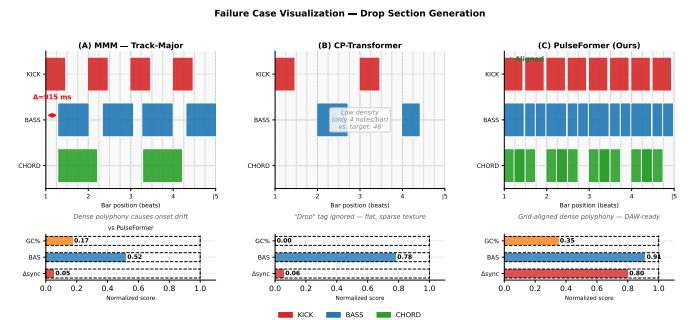
Fig. 5: Failure Case Visualization. (A) Track-Major models show large onset drift in dense passages. (B) The evaluated token-compression baseline lacks macro-structural tags and produces a flatter density profile. (C) The complete PulseFormer pipeline stacks dense polyphony on the DAW grid under explicit structural-density conditioning.
