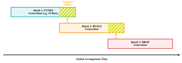
Fig. 3: Section-level scheduling pipeline. Each structural section is generated independently under its own \mathbf{E}_{level} prefix (structural density control identifier); the Temporal Anchor Stitching procedure concatenates sections at the engineering level. Structural density monotonicity across sections is a property of the external scheduler, not of the Transformer’s attention mechanism.
