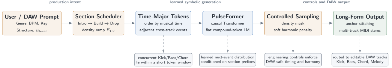
Fig. 1: Complete PulseFormer generation pipeline. Starting from user-supplied prefix conditioning (Genre, BPM, Key, Energy Level, Structure Tag), the system constructs a Time-Major interleaved token sequence, passes it through a 6-layer causal Transformer with a flat causal LM head over compound event tokens, applies dual algorithmic masks (Energy Density and Diatonic Scale), generates each structural section independently, and stitches all sections into a coherent multi-minute arrangement via Temporal Anchor Offset alignment.
